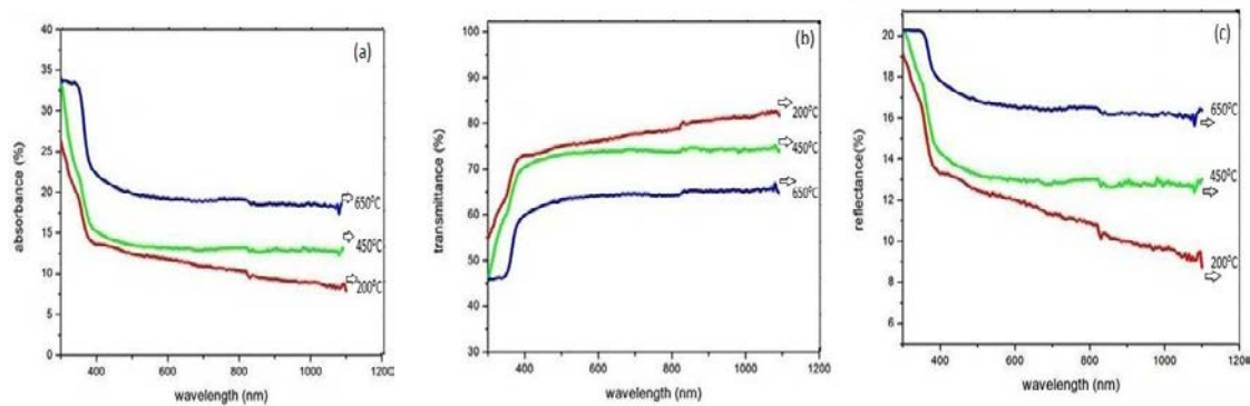
Fig. 2: (a) Graph between absorbance % and wavelength (nm). (b) Graph between transmittance % and wavelength (nm). (c) Graph between reflectance% and wavelength (nm), at various calcinations temperatures 200°C, 450°C and 650°C
