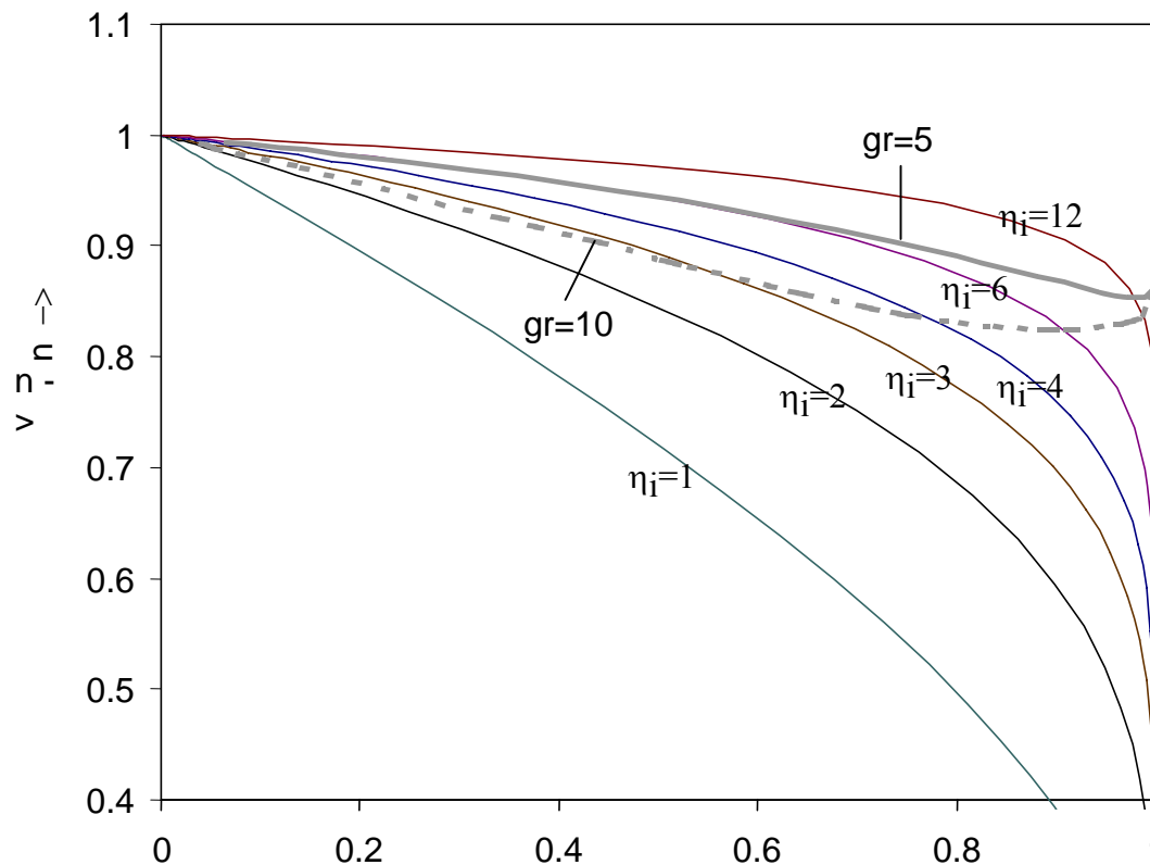
Fig. 6 Avrami exponents vs. fraction transformed for \eta_i = 1 to 12, as calculated from Eq. 3. Also presented are Avrami exponents for a one dimensional model representing the case of blocking resulting from anisotropic growth with growth rate anisotropy g_r = 5 and 10 (data from Ref. 37). Note that for a large range of \alpha values the latter data can be fitted well by Avrami exponents from Eq. 3.
