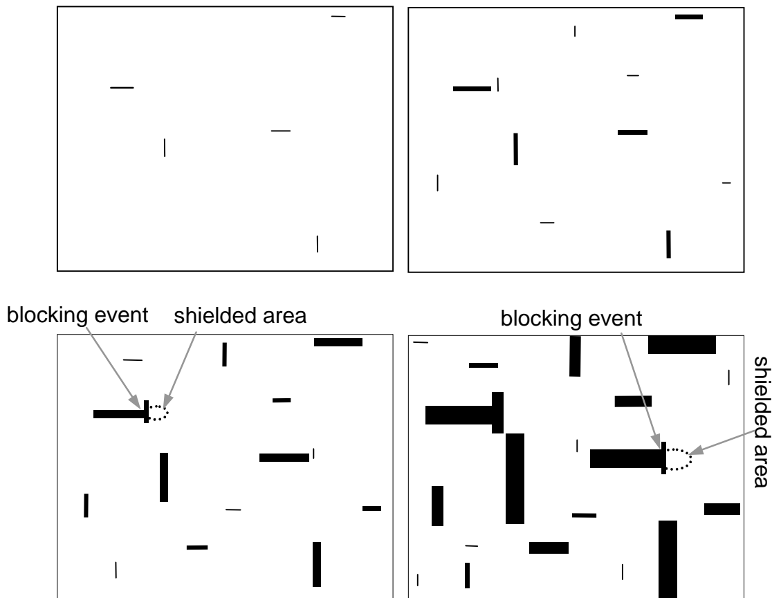
Fig. 5 Schematic illustration of blocking during the growth of anisotropic particles. The figure depicts a 2D transformation with nucleation and growth in which the growing particles are oriented normal to each other.
