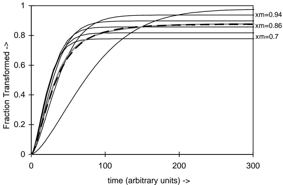
Fig. 4 Transformation curves for a reaction which is influenced by the Gibbs-Thomson effect. Presented are curves for various values of x_m .
