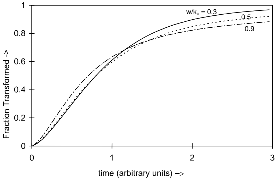
Fig. 1 Averaged fraction transformed for normally (Gaussian) distributed JMAK processes, with w/k_0 = 0.3, 0.5 and 0.9 , n = 1.5 .
