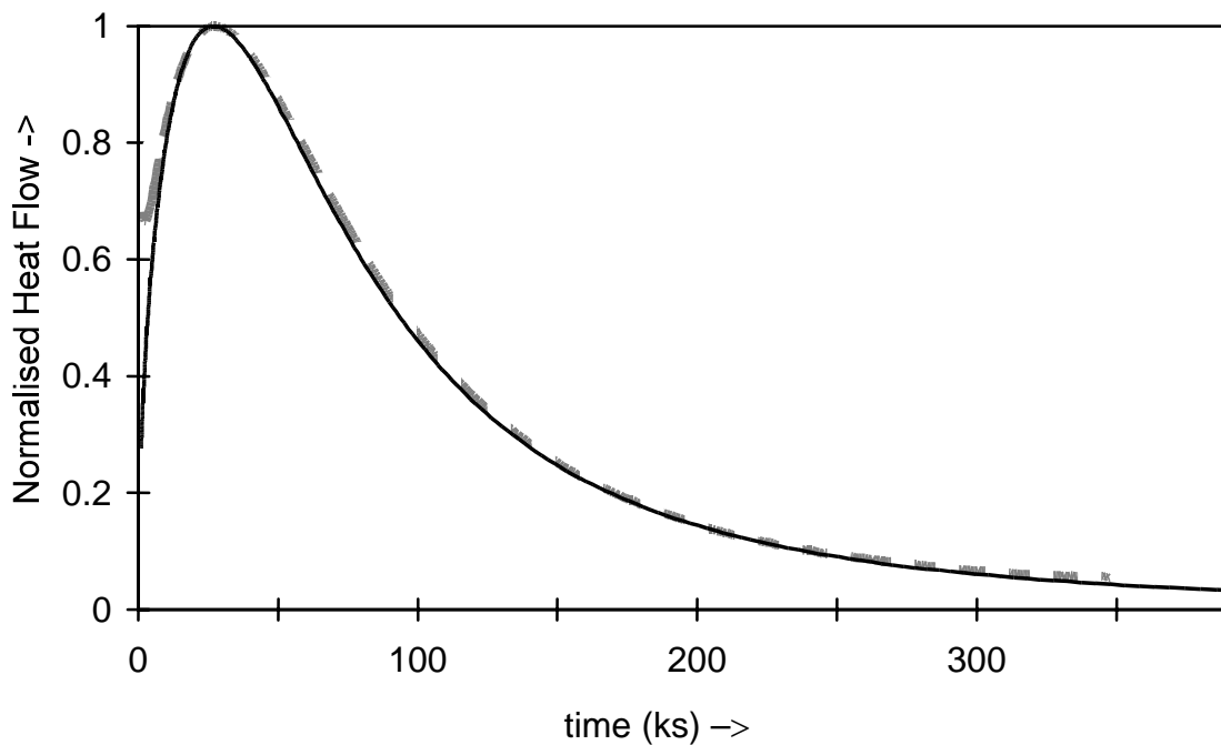
Fig. 7 Normalised heat flow curve for precipitation in air-cooled Al-6at%Si at 230°C (dashed grey line). The fit (thin, black line) is obtained with Eq. 3 and \eta_i = 1.1 , \eta_S = 1.5 .
