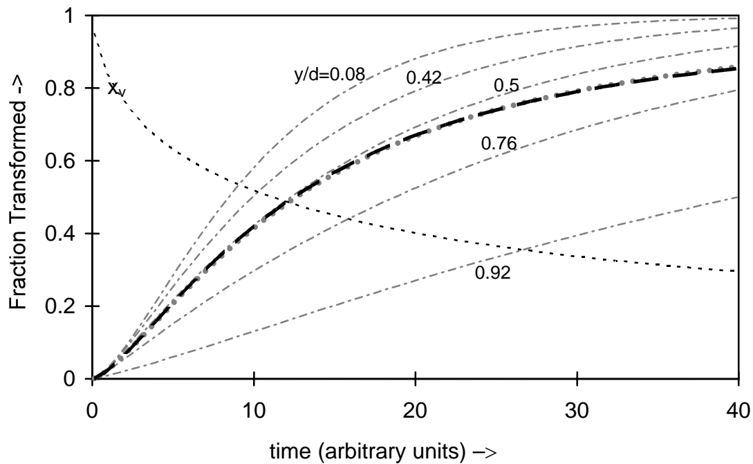
Fig. 3 Transformation curves for a reaction which is influenced by vacancy annihilation ( k_2/k_1 = 7 ). Presented are fractions transformed at various positions in the sample (---), the average fraction transformed (••••), and a fit of the latter based on Eq. 3 with \eta_i = 1.15 and n_S = 1.42 (— —). Also presented is the average concentration of vacancies remaining in the sample (•••).
