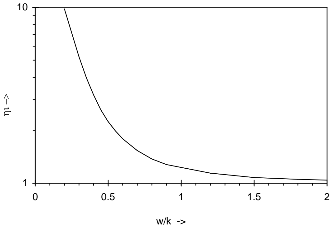
Fig. 2 Value of \eta_i for an optimal fit of Eq. 3 to averaged fraction transformed for normally (Gaussian) distributed JMAK processes, n = 1.5 (Fit is optimised for \alpha between 0 and 0.8)
