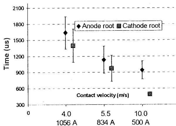
Fig. 8. Variation of contact velocity (m/s), with the associated current at contact opening.
