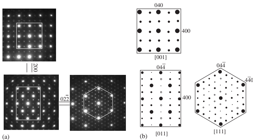
Fig. 2. (a) A series of SAD patterns tilted from one Nd-rich phase in the as-received sample; (b) Simulated diffraction patterns for Nd-rich phase based on the Ia\bar{3} structure ( \text{Mn}_2\text{O}_3 type) with lattice parameter a = 1.08\ \text{nm} . The solid and open circles represent real and double diffractions, respectively.
