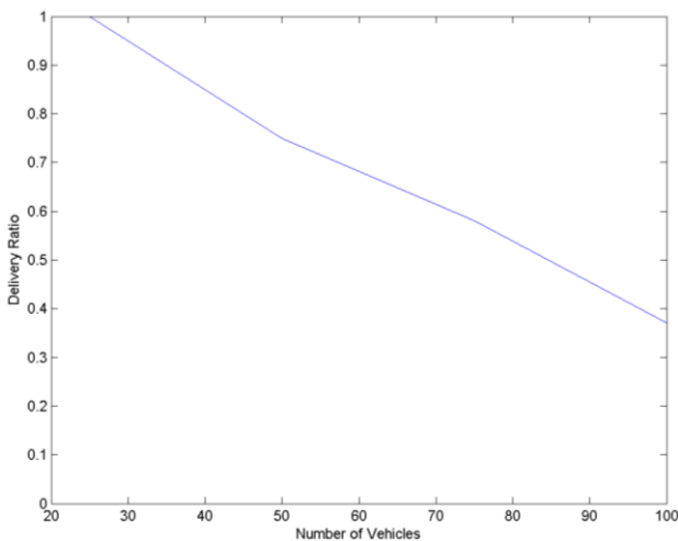
Figure 3. Delivery ratio
