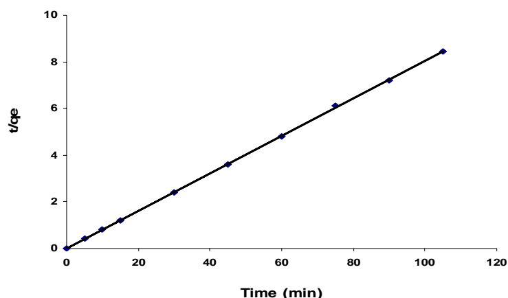
Fig. 7. Pseudo second-order adsorption kinetics of RB19 onto grapefruit peel; pH 2, 25 °C, Initial dye conc. of 50 mg L -1 and rate of 180 rpm.
