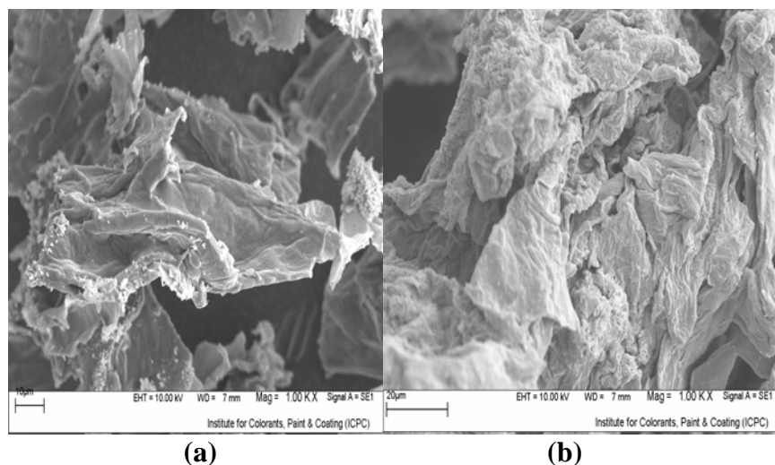
Fig. 6. Scanning electron micrographs of (a) original grapefruit peel, (b) dye adsorbed grapefruit peel with RB19. conditions: pH 2, 0.5 g in 150 ml of adsorbent, 50 mg L -1 of initial dye concentration, equilibrium time of 45 min, agitation rate of 180 rpm, 25 ± 1 °C and particle size of 150-ξ·0 µm.
