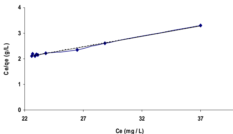
Fig. 5. Langmuir isotherm plot for reactive blue19 adsorption on waste grapefruit peel.
