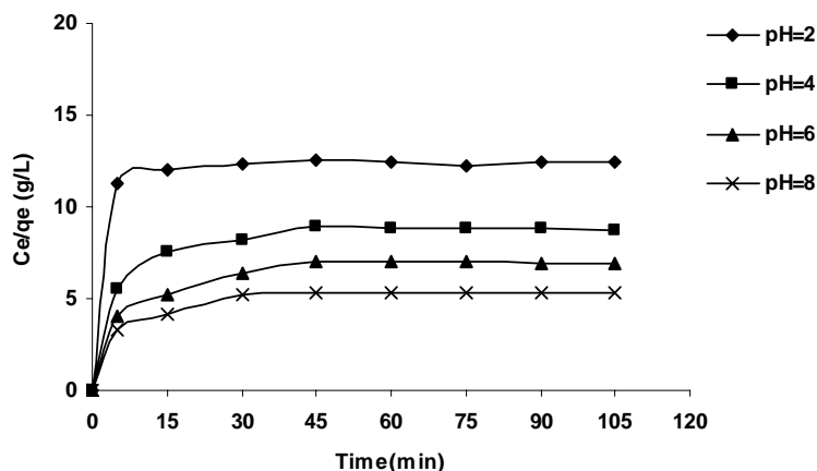
Fig. 3. Effect of pH on the removal of RB19; 45 min contact time, 25 °C, agitation rate of 180 rpm and 0.5 g adsorbent in 150 ml of 50 mg L -1 dye solution.
