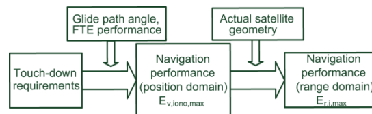
76 77 Fig. 2 Derivation of range-domain requirements from airworthiness considerations 78
