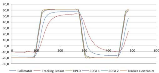
Figure 17: One temperature cycle during thermal vacuum test
