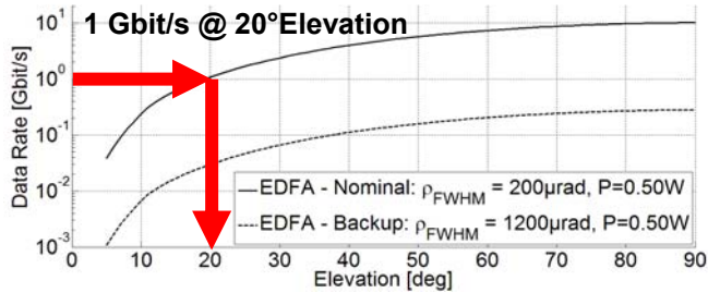
Figure 2: Link Budget (60 cm OGS @ DLR Oberpfaffenhofen, Atmospheric visibility: 22 km; Losses for atmospheric fading, the optical systems, tracking, etc. are included in the budget)
