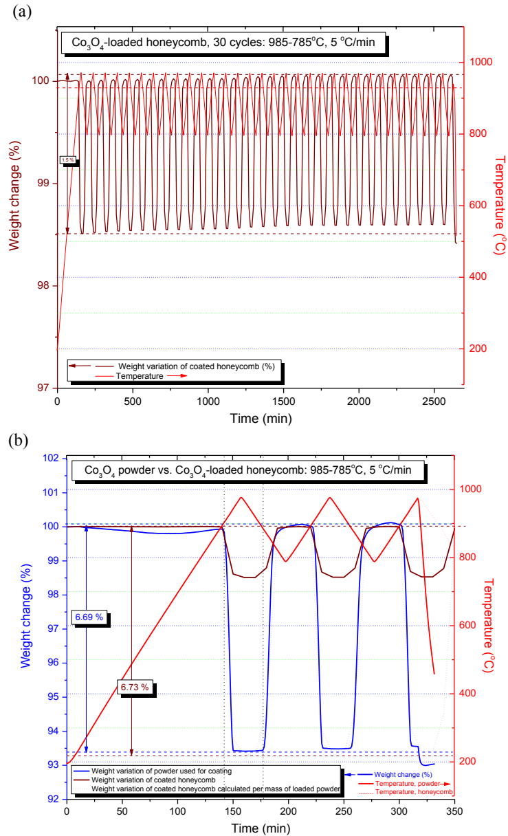
Fig. 4: (a) Thirty-cycles reduction/oxidation TGA test of mini-honeycomb loaded with 28 wt% Co 3 O 4 powder; (b) Comparison of weight variation as a function of temperature in the TGA between “plain” Co 3 O 4 powder and Co 3 O 4 -loaded honeycomb (first two redox cycles).
