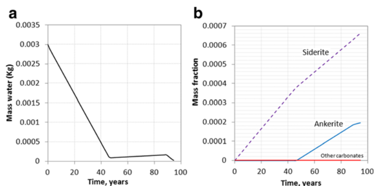
Figure 7 Basalt alteration in the scCO 2 rich phase with initial 3 grams of water per liter pore space. A) as zeolites form H 2 O is consumed and the water activity is reduced. After approximately 45 years most water is consumed, whereas all is gone before 100 years. B) siderite formed the secondary carbonate initially followed by ankerite.
