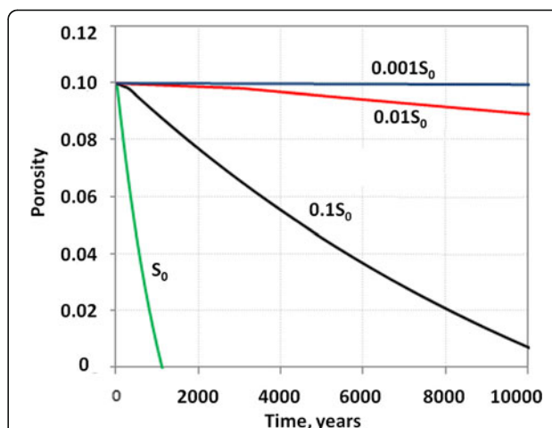
Figure 6 Porosity changes caused by the basalt alteration at 40 C and specific surface areas ranging from S 0 (estimated total basalt surface area) down to a three orders of magnitude reduction. The base case specific surface used was S 0 /10.
