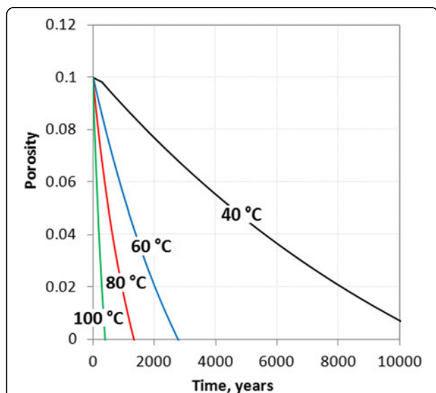
Figure 5 Porosity changes caused by the basalt alteration at 40 to 100 C. Secondary hydrated species and carbonates incorporate the H 2 O and CO 2 masses into the solids and clogs the pore space. As reaction rates increase exponentially with temperature, the pore space is filled up faster at the higher temperatures.
