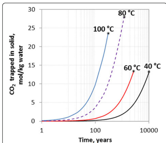
Figure 4 CO 2 trapped in solids for 40 to 100 C simulations at 100 bar CO 2 pressure. A cut-off value is used when all pore space is filled up with the secondary phases (see Figure 5). The simulations suggest that the total amount of secondary carbonates that form is dictated by the available pore space and the thermodynamic stability of secondary phases rather than temperature, whereas carbonate generation rates depend on the exponential increase of basalt dissolution rates with temperature.
