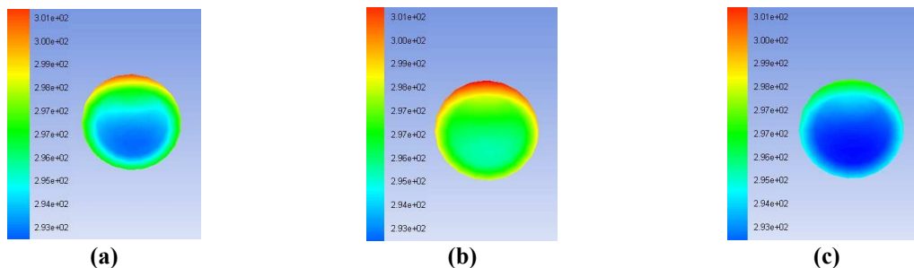
Fig. 5. Static temperature distribution within the middle riser pipe on (a) 15 th March (b) 15 th Jun (c) 15 th September under thermal loading of a working day
