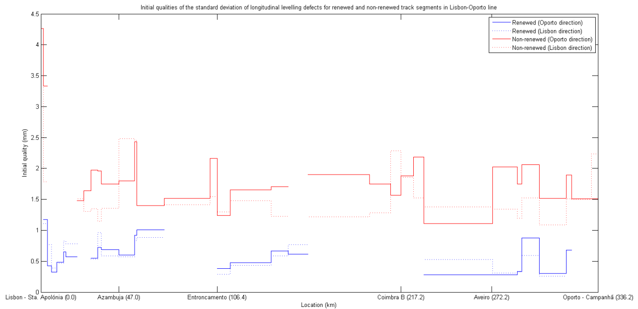
Figure 5 – Initial qualities of the standard deviation of longitudinal level defects for renewed ( \alpha ) and non-renewed ( \alpha' ) track segments in Lisbon-Oporto line.
