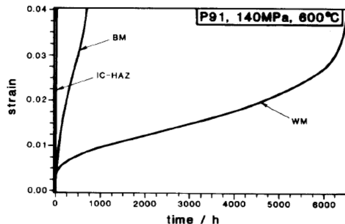
Fig.2. A strain-time creep curves for the three material states at 60°C and 140 MPa [5]
