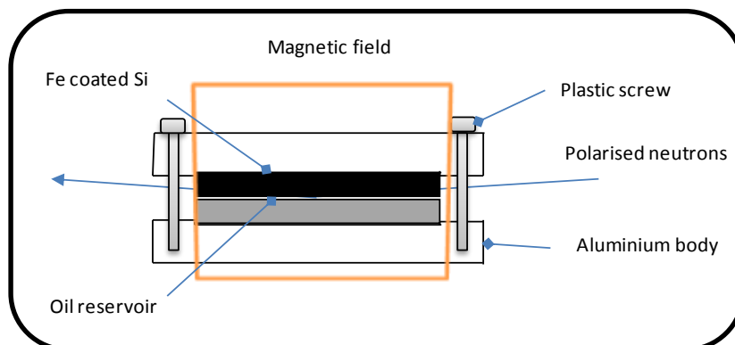
Figure 1. A schematic figure of the reflectivity cell used for the polarised neutron experiment.
