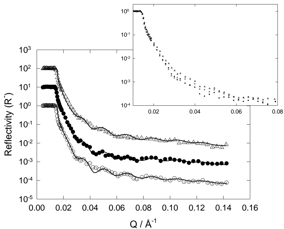
Figure 6. Reflectivity profiles for spin down neutrons for palmitic acid concentrations, 1000 ppm ( \Delta ), 500 ppm ( \bullet ) and 150 ppm ( \circ ) in d-hexadecane are shown. The fits to the data are shown by the solid lines. The fitted parameters are given in Table 2. The profiles are shifted by a factor of 10 for the purpose of clarity. The data is also shown (insert) on the same plot to highlight the changes in the reflectivity profiles as a function of concentration.
