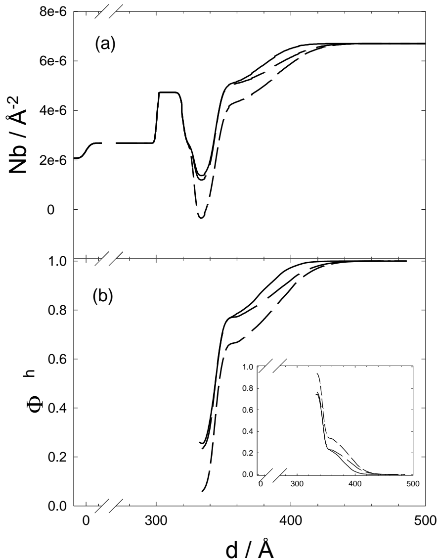
Figure 7(a). Scattering length density profiles for spin down neutrons for the palmitic acid in d-hexadecane. The introduction of a break in the scale is only to highlight the iron oxide/ oil interface. (b) Shows the volume fraction of hexadecane ( \Phi_h ) at the interface, whereas the volume fraction for palmitic acid ( \Phi_{PA}=1- \Phi_h ) is shown in the figure inset. Short dash line (150 ppm), dashed line (500ppm), solid line (1000ppp palmitic acid).
