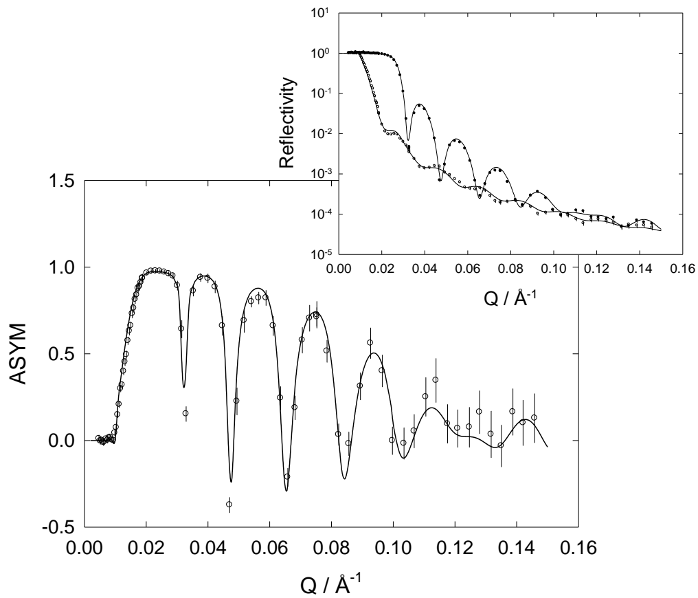
Figure 3. The spin asymmetry (ASYM) ((R^+ - R^-)/(R^+ + R^-)) for the substrate characterisation as a function of the scattering wave-vector ( Q ) is shown. The open circles are the data and the fit is shown by the solid line. The reflectivity profiles for spin up ( R^+ ) ( \bullet ) and spin down ( R^- ) ( \circ ) neutrons at the air/metal interface are shown as an insert. The solid lines correspond to the simultaneous fit to the data.
