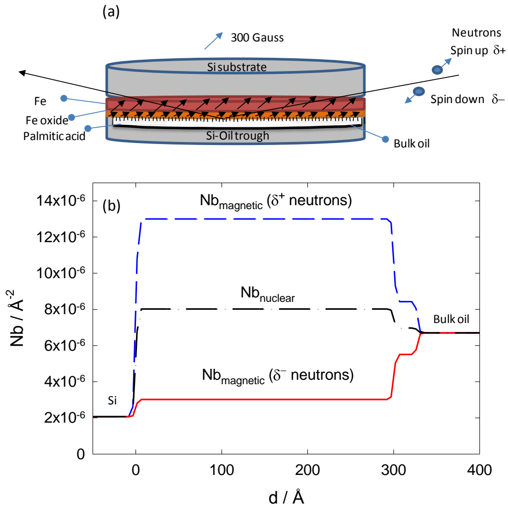
Figure 4. (a) A schematic figure of the experimental geometry used. (b) Idealised neutron scattering length density profiles of the iron coated Si in contact with d-hexadecane. The spin up neutrons (dashed line), spin down neutrons (solid line) and non-polarised neutrons (dashed-dotted line). The contrast using spin down neutrons minimises the reflection from the Si/iron interface, allowing the adsorption of palmitic acid onto the iron oxide/oil interface to be dominant.
