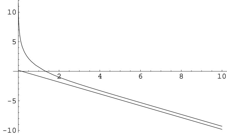
Figure 10: A plot of the logarithms of the LHS of (353) (top) against the RHS of (353) (bottom) against T for our chosen representations. We have in fact taken the N th root of each side. We can ignore the 3/\sqrt{8} factor on the RHS because it adds a small constant to the lower graph which does not affect the inequality for any value of N .
