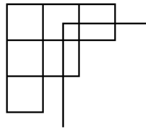
Figure 17: The elbow line for the box (1, 2) gives a hook length of 3.
