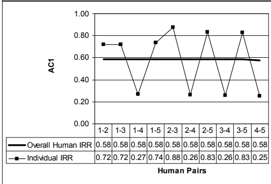
Figure 3 Inter-rater Reliability for Question 3
