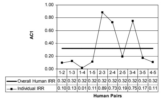
Figure 4 Inter-rater Reliability for Question 4
