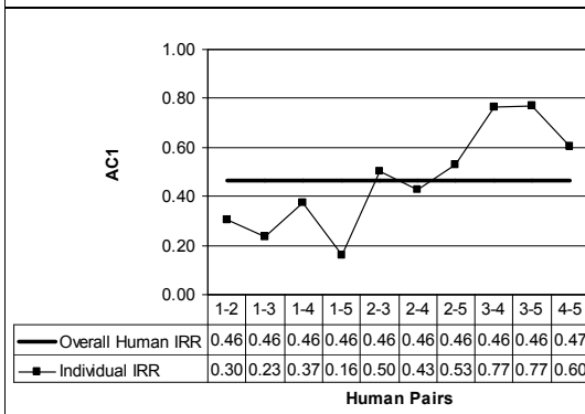
Figure 7 Inter-rater Reliability for Question 10
