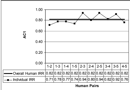
Figure 5 Inter-rater Reliability for Question 8
