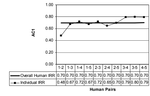
Figure 6 Inter-rater Reliability for Question 9
