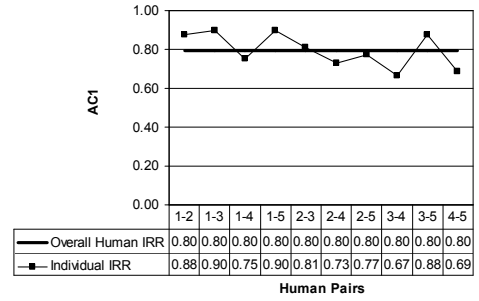
Figure 2 Inter-rater Reliability for Question 2
