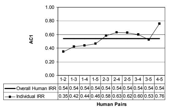
Figure 8 Inter-rater Reliability for Question 11
