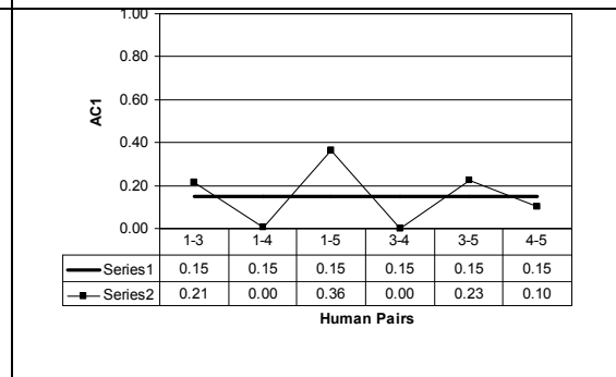
Figure 14 Inter-rater Reliability for Question 17
