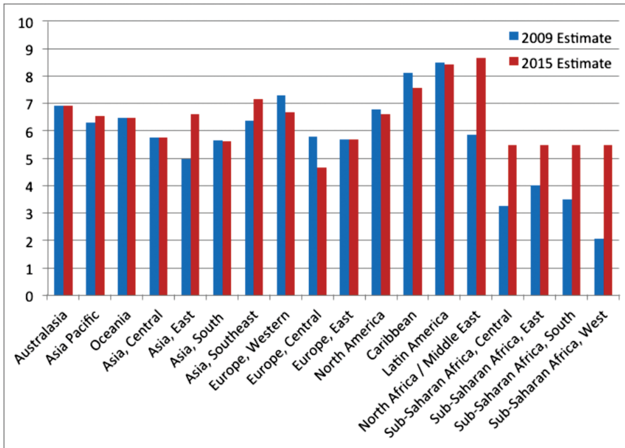
Figure 2.3 Estimated prevalence of dementia for those aged 60 and over, standardised to Western Europe population, by GBD region
