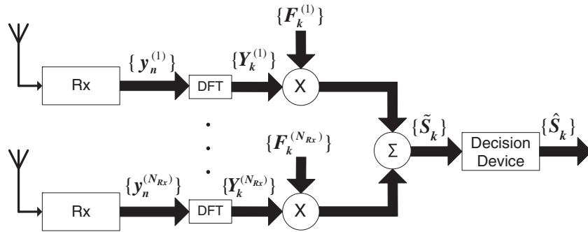
Figure 2. Orthogonal frequency division multiplexing receiver structure with an N_{Rx} -branch space diversity.
