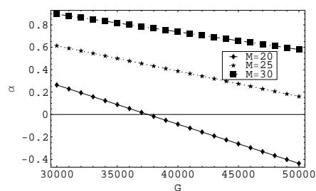
Figure 2.2: Fair \alpha - G combinations with parameters: r = 0.05 , g = 0.0275 , x = 35 , \sigma = 0.3 , K = 1000 and the other parameters are given in P12.
