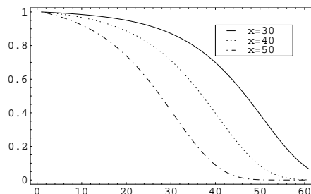
Figure 4.4: t p_x for x = 30, 40, 50 . The other parameters are given in Table 4.1
