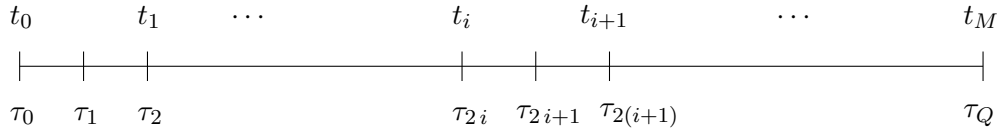
Figure 3.1: Partition of T according to premium payment dates ( \{t_0, t_1, \dots, t_{M-1}\} ) and trading dates ( \{\tau_0, \tau_1, \dots, \tau_Q\} ). Trading occurs e.g. twice as frequently as premium payments.
