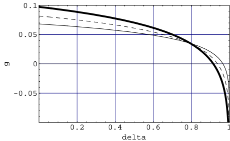
Figure 5.9: Relation between \delta and g for different \sigma with parameters (case (a)): A_0 = 100 ; L_0 = 80 ; \alpha = 0.8 ; r = 0.05 ; \eta = 0.8 ; T = 12 ; d = 1 ; \sigma = 80 ; \alpha = 0.8 ; r = 0.05 ; \eta = 0.8 ; \sigma = 0.2 ; d = 1 ; T = 0.15 (solid); \sigma = 0.20 (dashed); \sigma = 0.25 (thick). Figure 5.10: Relation between \delta and g for different T with parameters (case (a)): A_0 = 100 ; L_0 = 80 ; \alpha = 0.8 ; r = 0.05 ; \eta = 0.8 ; \sigma = 0.2 ; d = 1 ; T = 12 (solid); T = 18 (dashed); T = 24 (thick).
