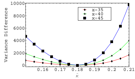
Figure 4.8: Variance difference as function of \tilde{\kappa} with the real \kappa = 0.18 for \tilde{x} = 35 , \tilde{x} = 40 and \tilde{x} = 45 . The other parameters are given in Table 4.1.
