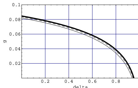
Figure 5.3: Relation between \delta and g for different \eta with parameters (case (a)): A_0 = 100 ; L_0 = 80 ; \alpha = 0.8 ; r = 0.05 ; \sigma = 0.2 ; T = 12 ; d = 1 ; \eta = 80 (solid); \eta = 0.8 (dashed); \eta = 0.9 (thick). Figure 5.4: Relation between \delta and g for different d with parameters (case (a)): A_0 = 100 ; L_0 = 80 ; \alpha = 0.8 ; r = 0.05 ; \eta = 0.8 ; \sigma = 0.2 ; T = 12 ; d = 0.5 (solid); d = 1 (dashed); d = 2 (thick).
