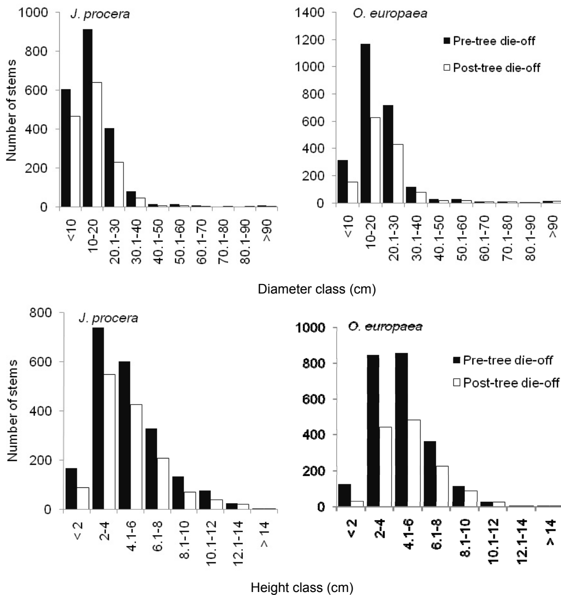
Figure 6.7 Diameter and height distribution of J. procera and O. europaea subsp. cuspidata with snags (pre-tree dieback) and without snags (post-tree dieback) in a dry Afromontane forest, northern Ethiopia.
