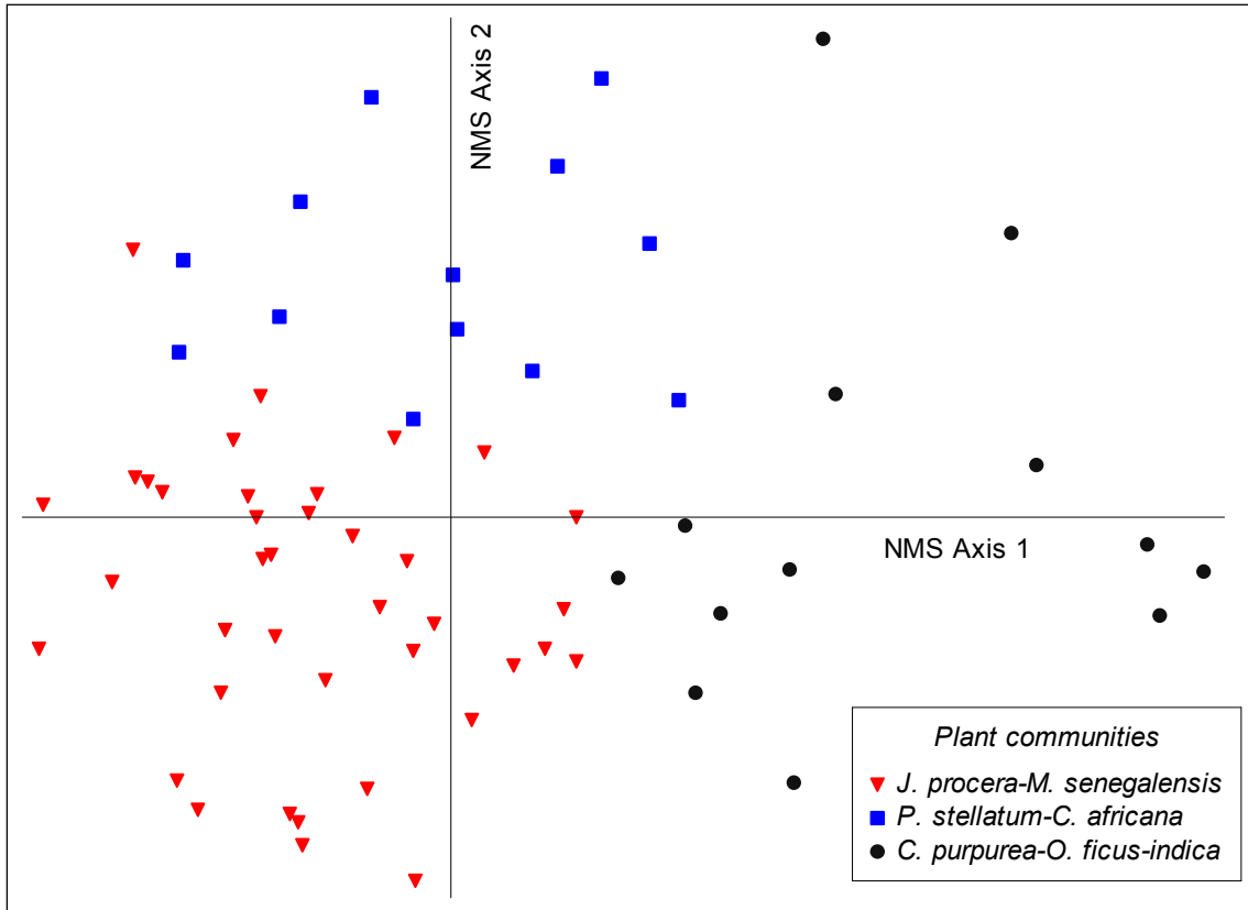
Figure 4.3 Nonmetric multidimensional scaling (NMS) ordination of the 65 plots in Hugumburda forest, northern Ethiopia.
