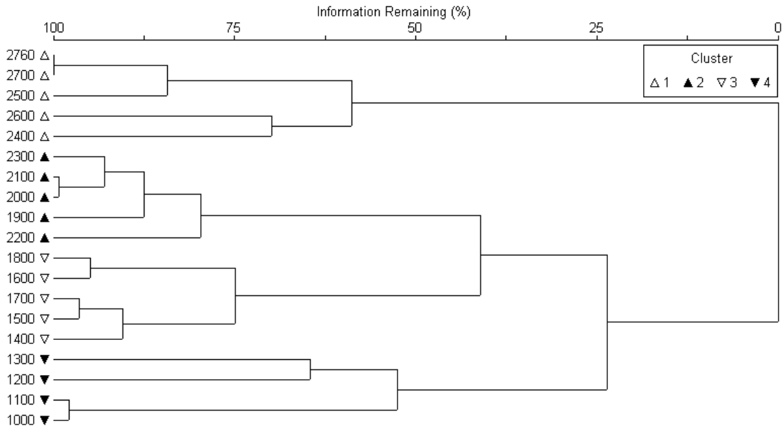
Figure 5.5 Dendrogram of the hierarchical cluster analysis of sampling points taken along an elevational gradient on the western escarpment of the Great Rift Valley, northern Ethiopia. By cutting the dendrogram at the 53 % information remaining level, four distinctive plant communities along the 1760 m elevation gradient were identified (C1: 2760, 2700, 2600, 2500, 2400; C2: 2300, 2200, 2100, 2000, 1900; C3: 1800, 1700, 1600, 1500, 1400; C4: 1300, 1200, 1200, 1100).
