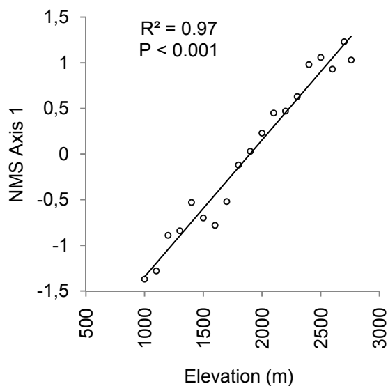
Figure 5.9 Relationship between elevation and NMS axis 1, on the western escarpment of the Great Rift Valley, northern Ethiopia.
