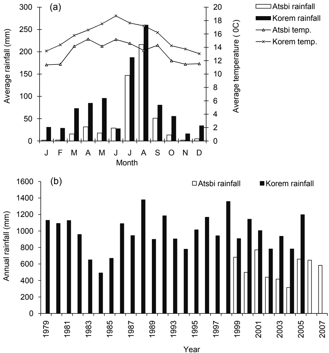
Figure 3.3 (a) Mean monthly rainfall and mean monthly temperature, and (b) annual rainfall recorded at Atsbi (Desa'a forest) and at Korem meteorological station (Hugumburda forest), northern Ethiopia.
