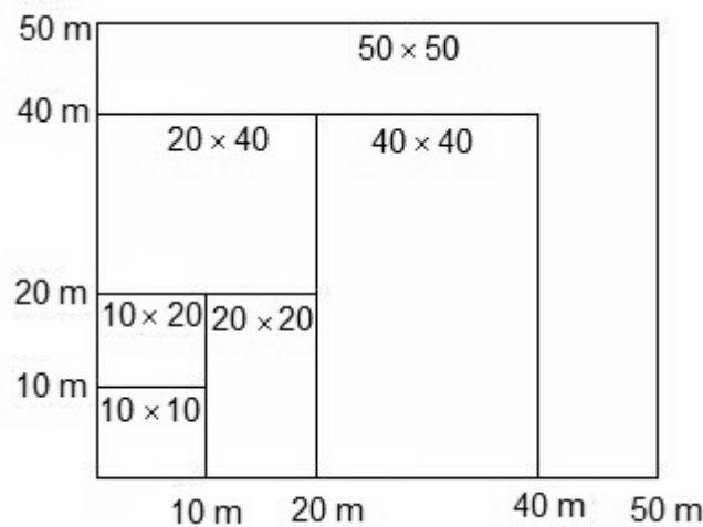
Figure 3.6 Layout of a nested plot used in vegetation data collection.
