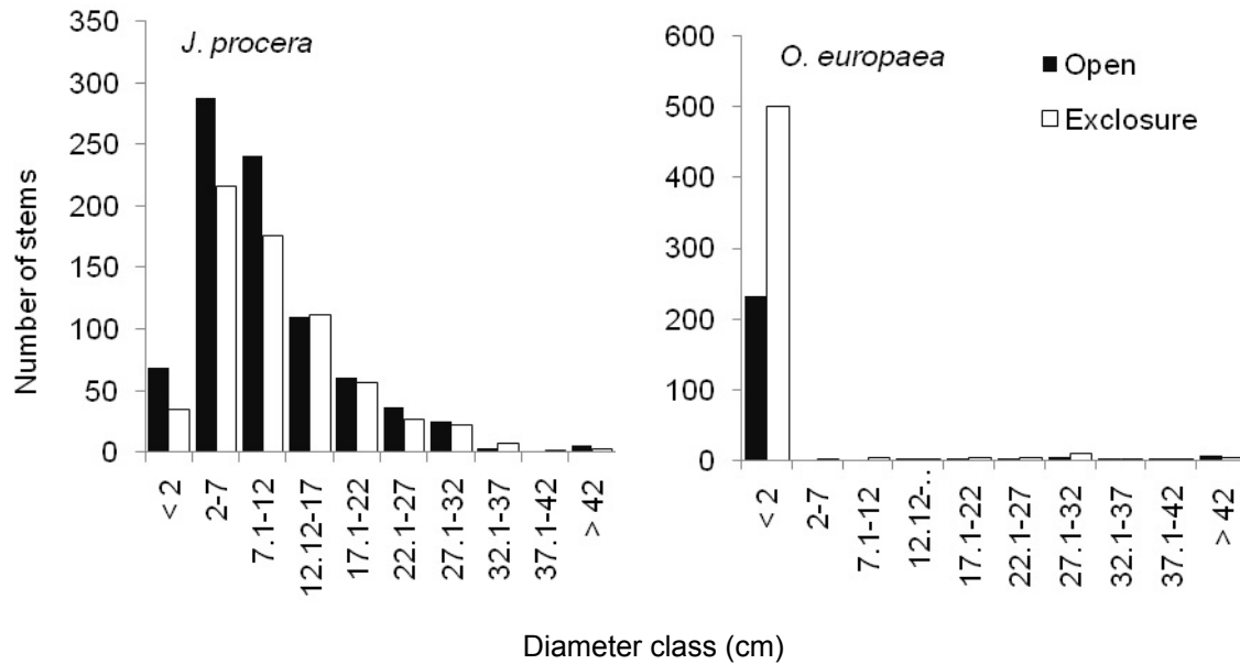
Figure 7.2 Diameter (DBH) class distribution of Juniperus procera and Olea europaea subsp. cuspidata in an exclosure and open forest in northern Ethiopia.
