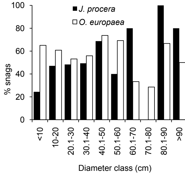
Figure 6.8 Percentage of snags according to stem diameter class in a dry Afromontane forest, northern Ethiopia.
