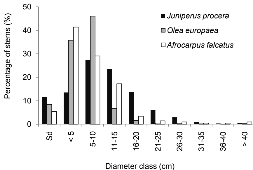
Figure 4.6 Diameter class distribution of the three native tree species in Hugumburda forest, northern Ethiopia. Sd = seedling.
