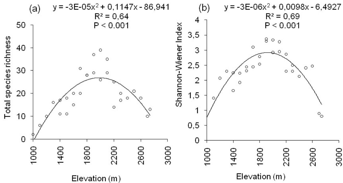
Figure 5.3 Patterns of species richness (a) and diversity (b) along an elevational gradient in the western escarpment of the Great Rift Valley, northern Ethiopia.
