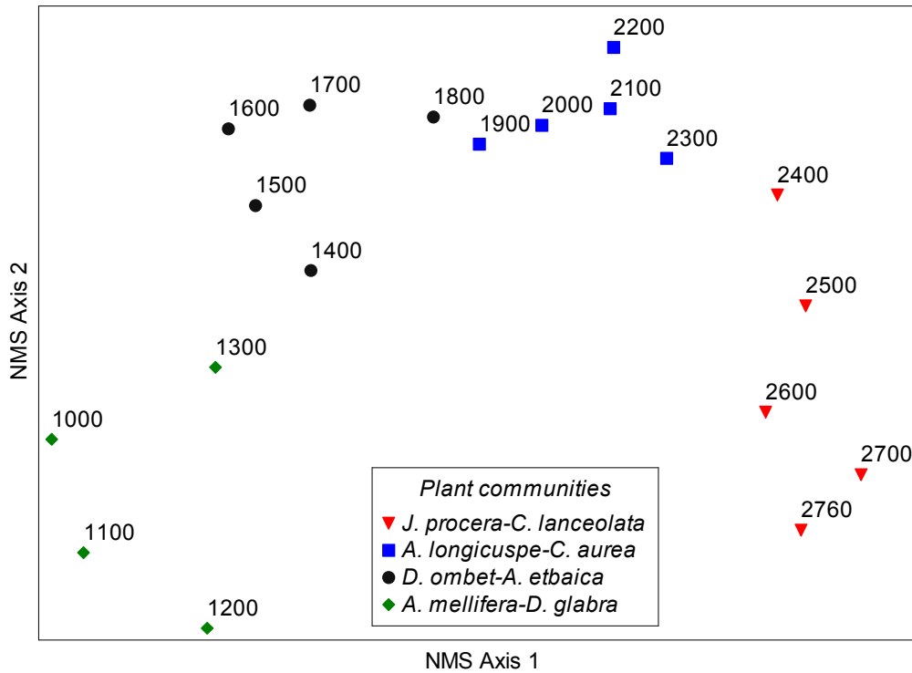
Figure 5.8 Nonmetric multidimensional scaling (NMS) ordination bi-plot showing the composition of plant communities along elevational gradient on the western escarpment of the Great Rift Valley, northern Ethiopia. Numbers indicate elevations labeled into the four groups derived by cluster and indicator species analyses.
