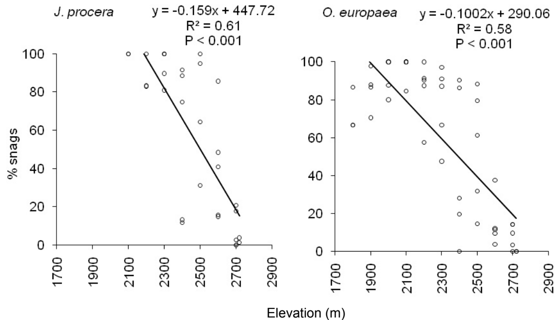
Figure 6.3 Percentage of snags of Juniperus procera and Olea europaea subsp. cuspidata along an elevation gradient in a dry Afromontane forest, northern Ethiopia.
