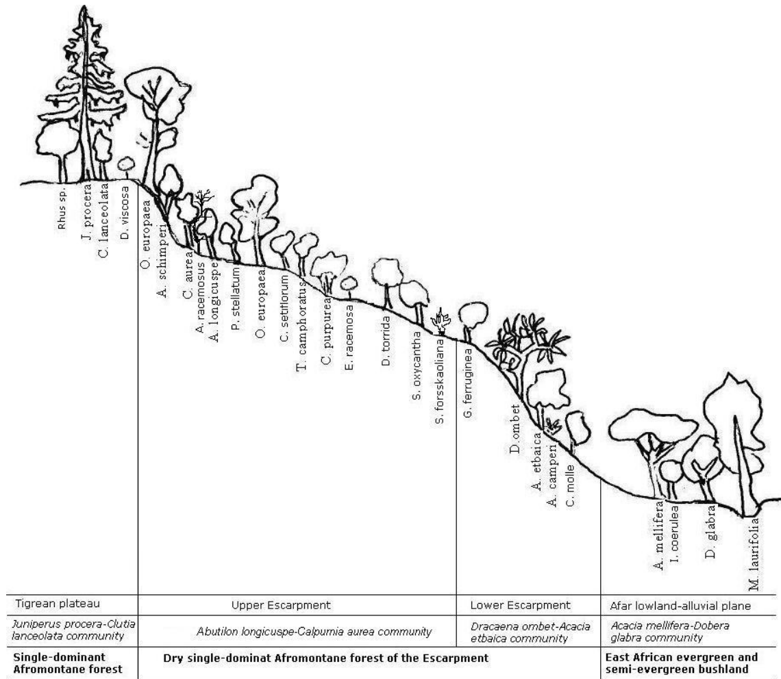
Figure 5.6 Vegetation profile along elevational gradient on the western escarpment of the Great Rift Valley, northern Ethiopia.
