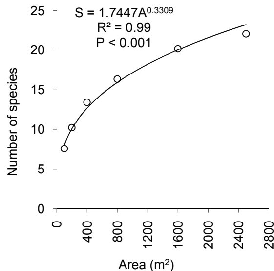
Figure 4.2 Species-area relationship at Hugumburda forest, northern Ethiopia.
