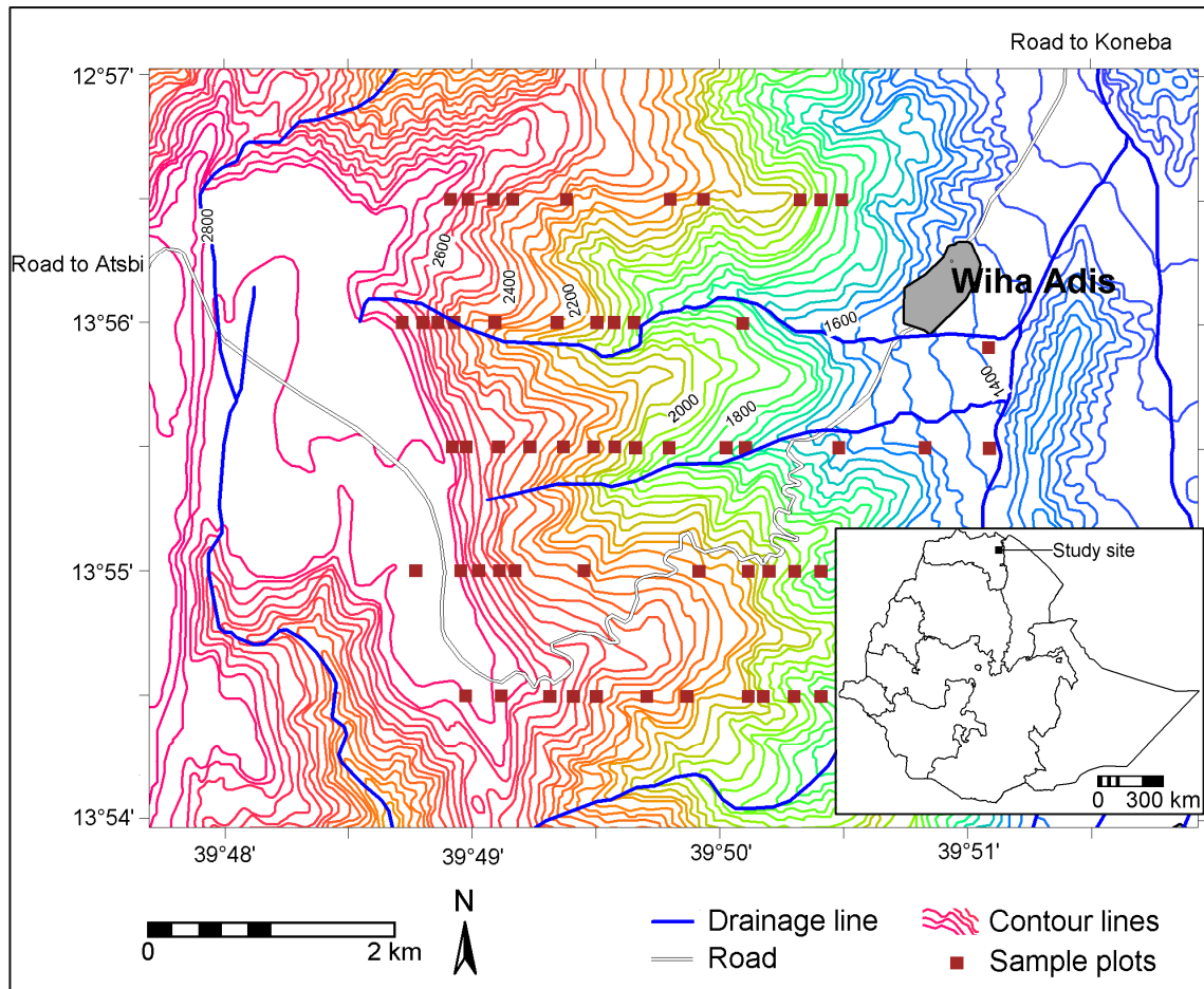
Figure 6.1 Location of the study area indicating the 57 sampling plots on a contour background map.
