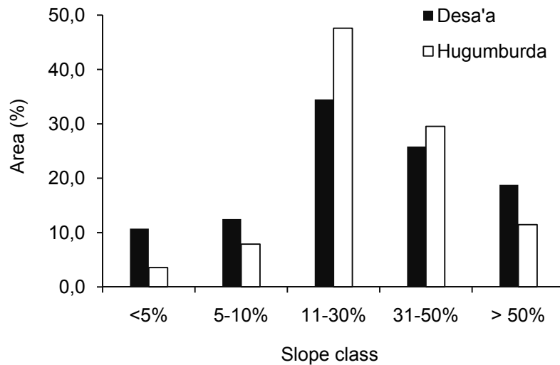
Figure 3.2 Slope classes distribution in Desa'a and Hugumburda forests, northern Ethiopia.
