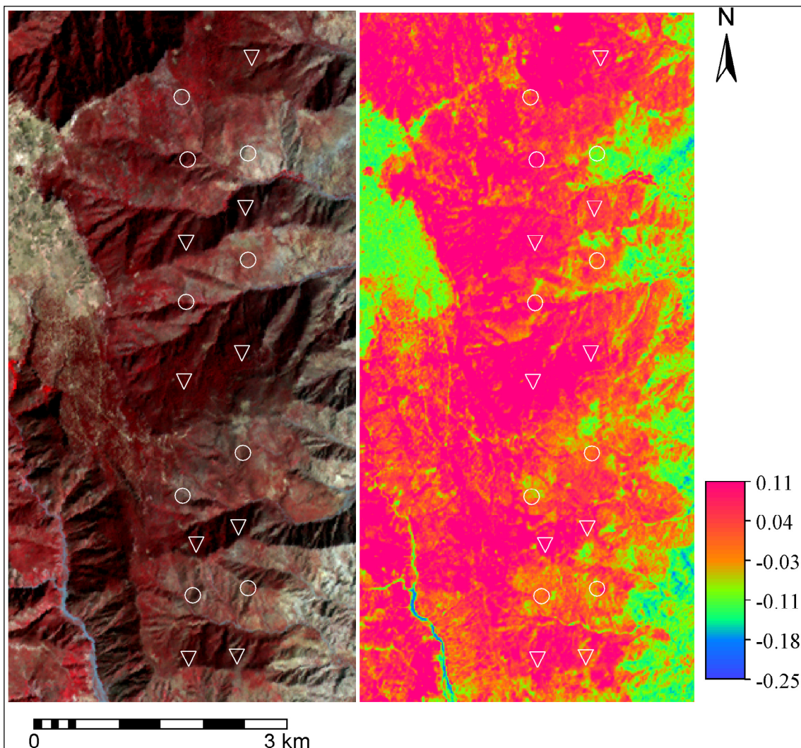
Figure 6.5 False Colour Composite (left) and NDVI map of ASTER imagery (right) showing low (▽) and high (o) extent of tree die-off (percentage snags per plot) along a micro-topography in a dry Afromontane forest, northern Ethiopia.
