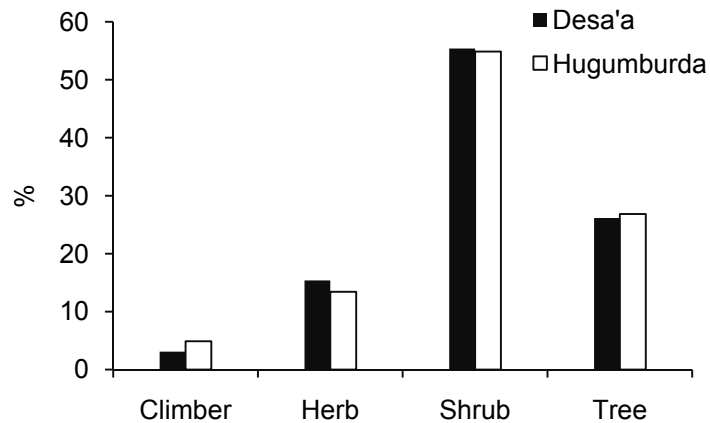
Figure 3.4 Life forms in Desa'a and Hugumburda forests, northern Ethiopia.
