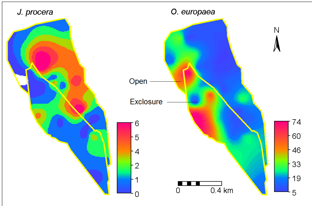
Figure 7.3 Kriged maps showing spatial distribution of seedling density of Juniperus procera and Olea europaea in the exclosure and in the open-access forest in northern Ethiopia. Numbers in the legend indicate the number of seedlings per plot (10 m × 10 m).
