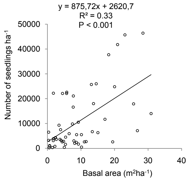
Figure 4.5 Relationship between basal area and seedling density in Hugumburda forest, northern Ethiopia.
