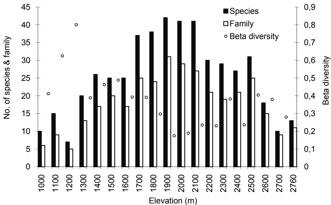
Figure 5.4 Trends in \alpha - and \beta -diversities along an elevational gradient on the western escarpment of the Great Rift Valley, northern Ethiopia. Species turnover between adjacent elevations is based on the Wilson and Shmida's \beta -diversity.
