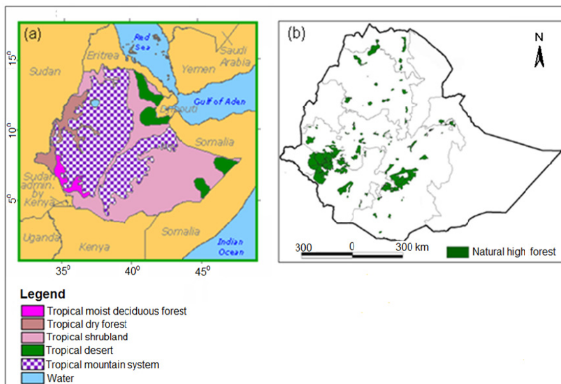
Figure 2.2 Ecological zones (a) (Map source: FAO 2001) and the fragmented natural high forests (b) (Map source: Ministry of Agriculture 2003) in Ethiopia.
