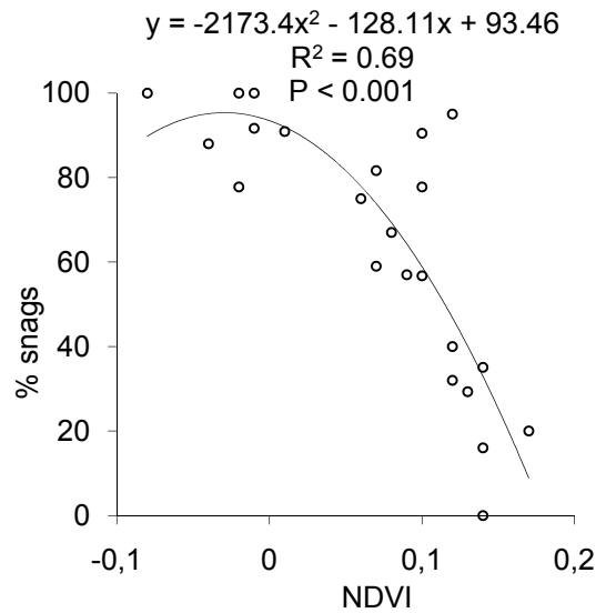
Figure 6.6 Relationship between mass tree dieback (per cent snag per plot) and NDVI along micro-topography in a dry Afromontane forest, northern Ethiopia.
