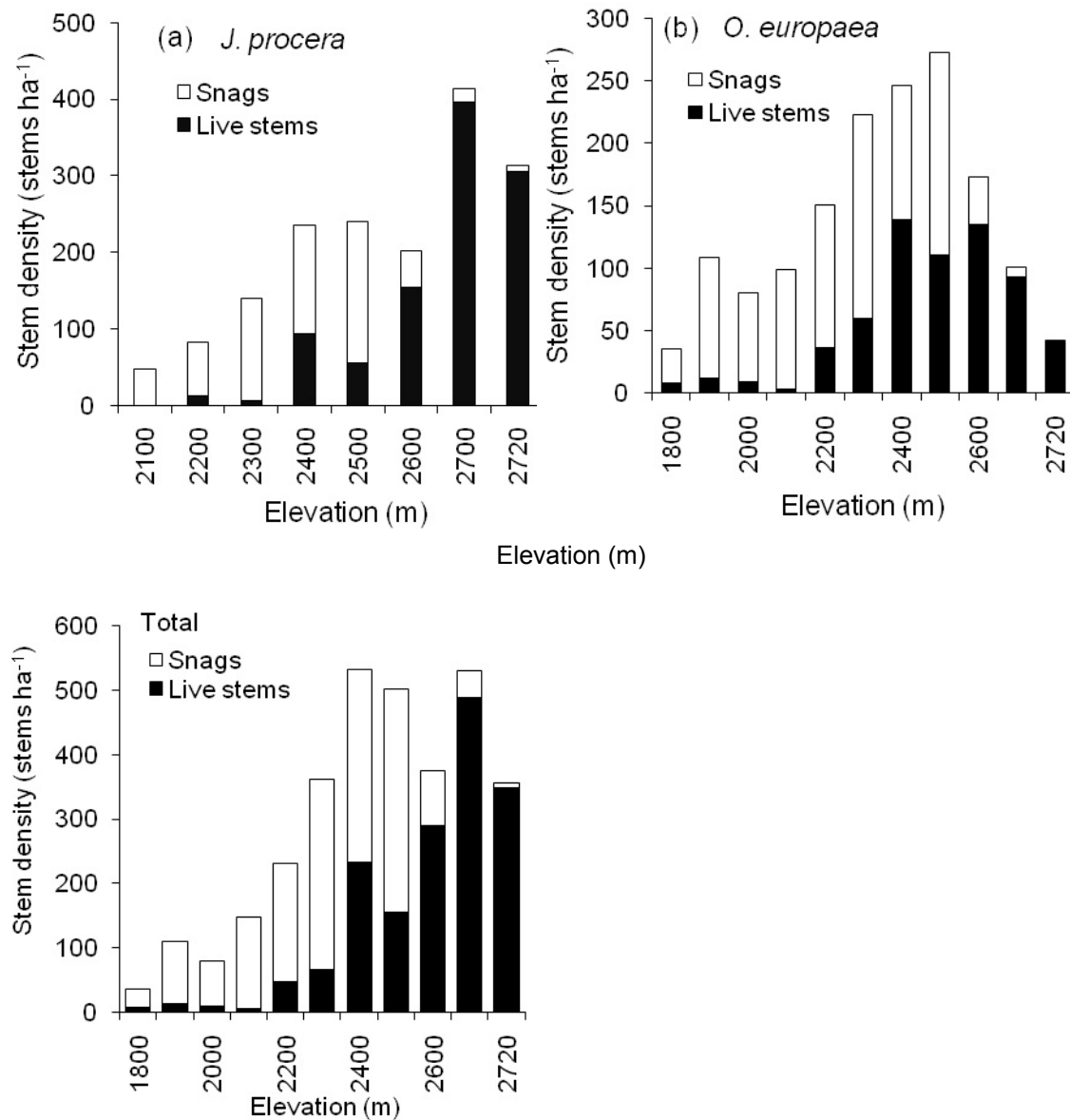
Figure 6.2 Mean densities of live stems and snags of Juniperus procera , Olea europaea subsp. cuspidata , and total (pooled data of the two species) along an elevational gradient in a dry Afromontane forest, northern Ethiopia.
