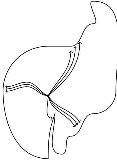
FIGURE 3. A domain with a spike in the interior: the geodesics in the Croke-Dzérdinski inequality take notice but are not as sensitive to its presence as other quantities (say, the inradius).
