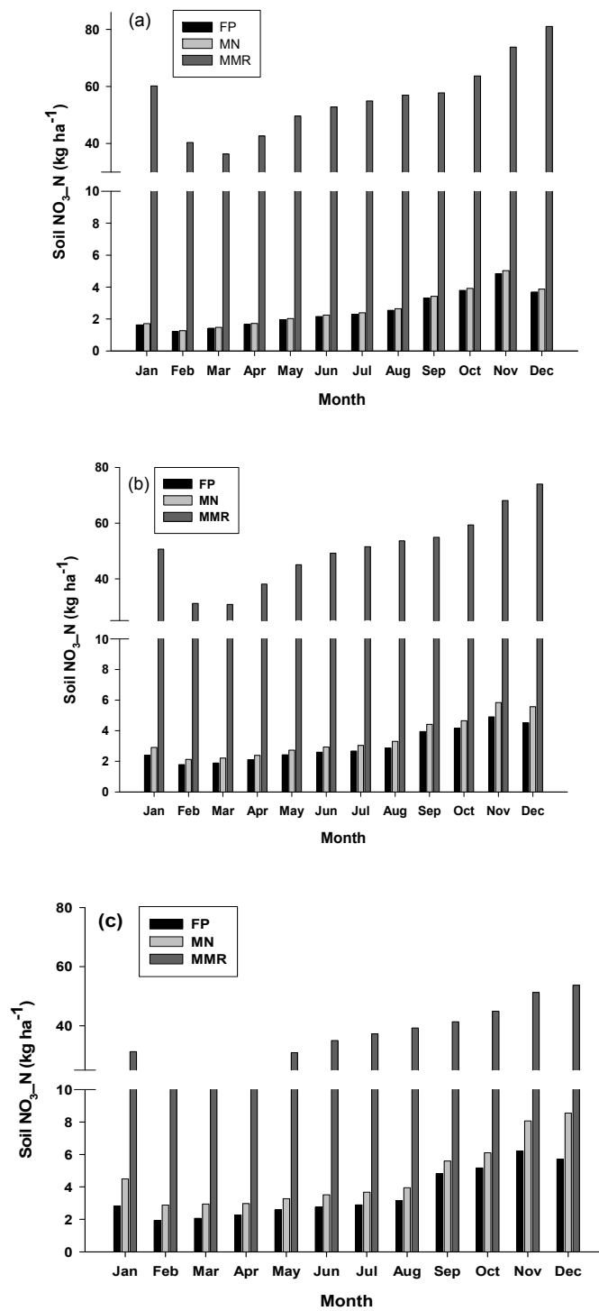
Figure 5.5 a-c Soil nitrate nitrogen (NO 3 -N) averaged for each month for the simulated 30 years for the farmer wealth categories (a), poor, (b) average, and (c) better-off. FP = farmer practice, MN = manure, MMR = maize-mucuna rotation.
