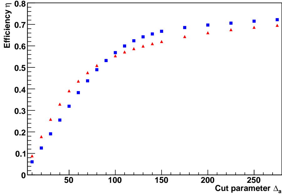
Figure 38: Reduction of reconstructed hits in dependency of the cut parameter \Delta_a - the maximal accepted difference between x and y total cluster energy. \eta = \# \text{ reconstructed hits} / \# \text{ combinatorial hits} . (Red triangles = GEM1, blue squares = GEM2).
