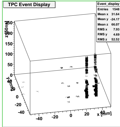
Figure 44: A double track along the z axis from the electron beam can be observed. The amplitudes are almost identical with a frame, which is an indication for cross talk.
