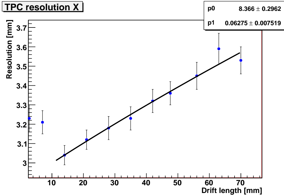
Figure 50: Resolution in x projection in dependency of the z coordinate of the primary ionization. Including a fit of the s_x(z) function on the data points.
