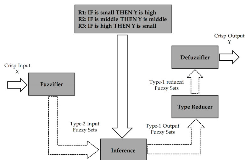
Figure 7. The proposed fuzzy type-2 scheme for the FMEA.
