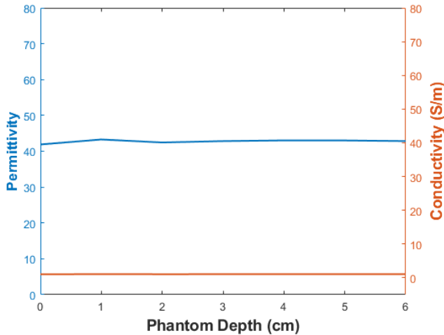
Fig. 3: Dielectric properties of 6.5cm thick phantom measured at seven different depths by increment of 1cm from surface to inside at 500MHz.
