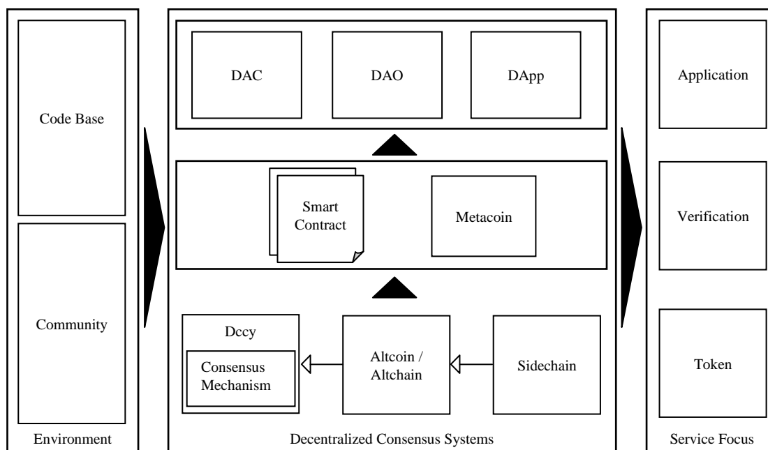
Figure 1. Overview of decentralized consensus systems and their relationships.
