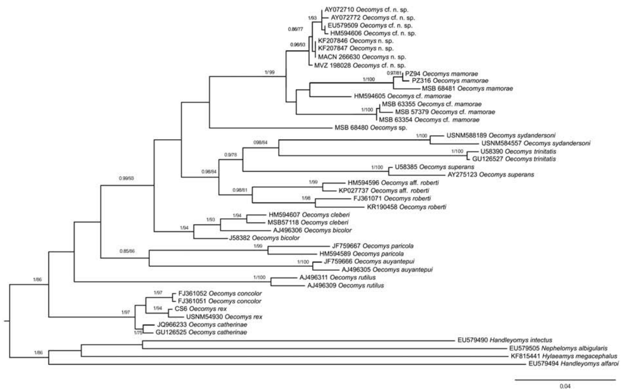
Fig. 1. —Maximum likelihood (ML) analysis of cytochrome- b sequences for 42 ingroup terminals and 4 individuals representing outgroup taxa (GTR+I+ \Gamma_6 , ln-likelihood = -5573.75833 ). Node support includes Bayesian posterior probabilities (only values equal or above 0.85) to the left of the diagonal and percentages of 1,000 bootstrap replicates (values above 75%) after the diagonal for nodes recovered in common by ML and BI analyses. GenBank access codes or specimen identification numbers correspond to those of Table 1.
