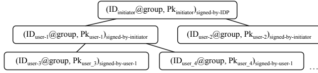
Figure 9: Access graph for group membership.
