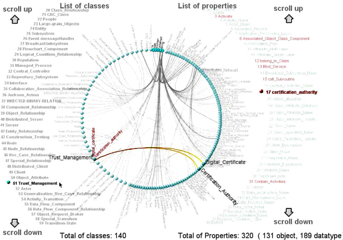
Fig. 8. The global coupling visualization shows the relations among classes in the ontology. The class “Trust_Management” has been selected as well as its coupled classes “Digital_Certificate” and “Certification_Authority”.
