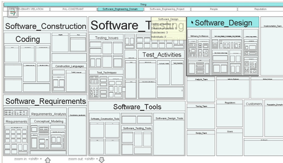
Fig. 5. The treemap represents the hierarchy of the ontology SEOntology. The class “Software_Design” has been highlighted, and its superclass “Software_Engineering_Domain” is also highlighted.
