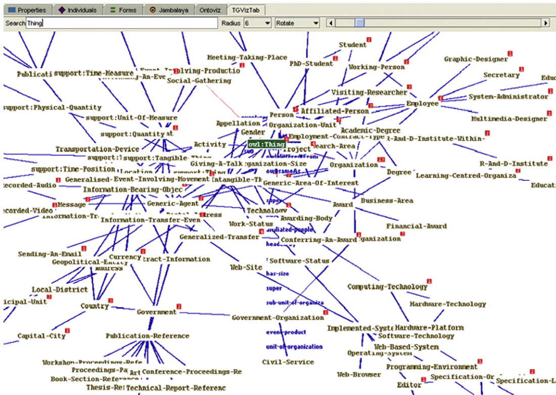
Fig. 4. The Protégé TGVizTab visualization based on the use of directed graphs. The main problems with this visualization are the occlusion and the overcrowding of visual elements.
