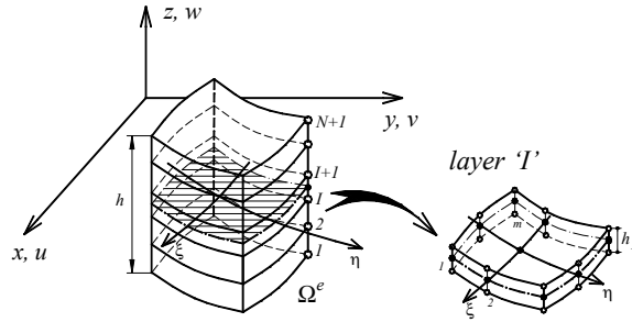
Figure 1. Plate finite element with n layers and m nodes
