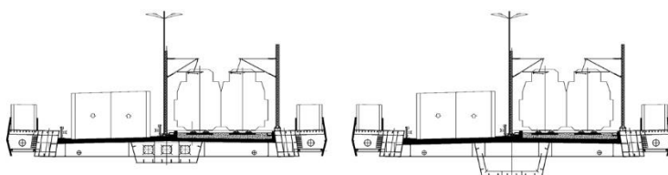
Fig. 8: Cross-sections of approach spans 1-2 and 4-5
