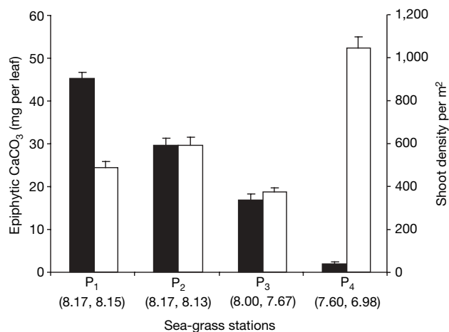
Figure 3 | Sea-grass shoot density and amount of epiphytic \text{CaCO}_3 on leaves growing at differing pH levels south of Castello d'Aragnese. Shoot density (open column, n = 4 , mean and s.d.) and epiphytic \text{CaCO}_3 (filled column, n = 80 , mean and s.d.) for data from 18 April to 9 May 2007 at various pH levels (mean and minimum values are shown; P_1 n = 30 , P_2 n = 16 , P_3 n = 23 and P_4 n = 37 ).
