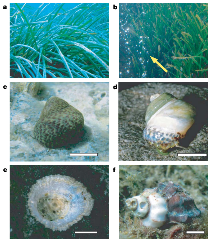
Figure 4 | Dissolution of calcified organisms due to naturally acidified sea water. a , Posidonia oceanica with heavy overgrowth of Corallinaceae at pH 8.2 ( a ) and lacking Corallinaceae at mean pH 7.6 ( b ); arrow indicates bubbles from the \text{CO}_2 vent field. c , d , Typical examples of O. turbinata with the periostracum intact at pH 8.2 ( c ) and with old parts of the periostracum removed at mean pH 7.3 ( d ). e , f , Live P. caerulea ( e ) and H. trunculus ( f ) showing severely eroded, pitted shells in areas of minimum pH 7.4. Scale bars represent 1 cm.
