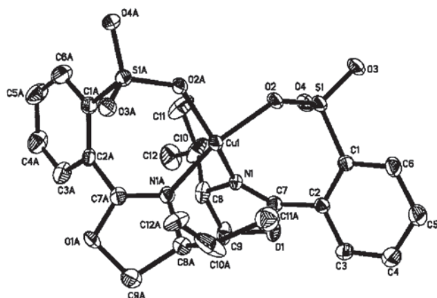
Figure 4. Molecular structure of 8 . Selected interatomic distances (Å) and angles ( ^{\circ} ) Cu(1)–O(2) 1.940(3), Cu(1)–O(2a) 1.946(3), Cu(1)–N(1) 1.947(4), Cu(1)–N(1A) 1.942(3), O(2)–Cu–O(2A) 86.80(12), O(2)–Cu–N(1) 96.03(13), O(2A)–Cu–N(1A) 94.18(13), N(1)–Cu–N(1A) 92.13(14), O(2)–Cu–N(1) vs. O(2A)–Cu–N(1A) interplanar twist angle 31.4^{\circ} .
