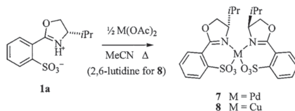
Scheme 3. Preparation of metal complexes of 1a .
