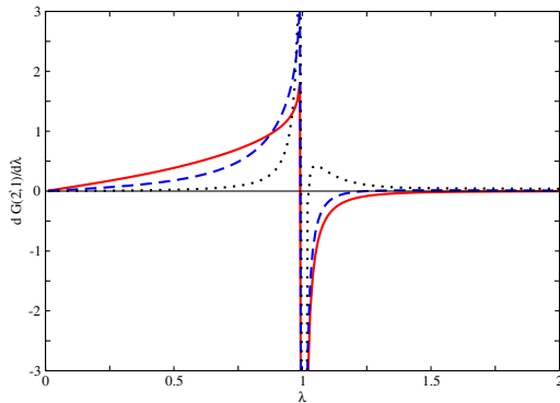
FIG. 2 (color online). Derivative of the lower bound of \mathcal{G}(2, 1) for three values of anisotropy: \gamma = 1 (red solid line), 0.6 (blue dashed line), and 0.2 (black dotted line). The second phase transition is also imprinted for the \gamma = 0.2 as the curve crosses the abscissa at \lambda = 1/\sqrt{1 - \gamma^2} .
