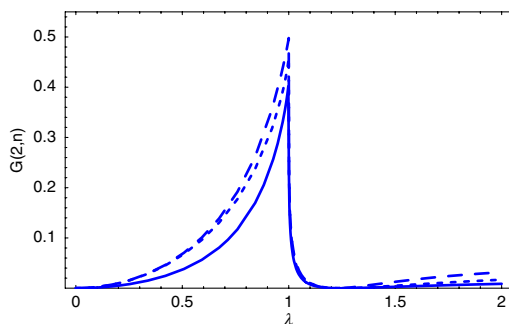
FIG. 3 (color online). Lower bound of \mathcal{G}(2, n) for \gamma = 0.6 and for three values of n : n = 1 (solid line), 2 (dashed line), and 7 (long-dashed line).
