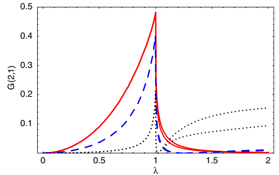
FIG. 1 (color online). Upper and lower bounds of \mathcal{G}(2, 1) for the XY chain for three values of the anisotropy: \gamma = 1 (red solid line), 0.6 (blue dashed line), and 0.2 (black dotted line).
