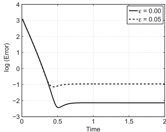
Fig. 12. Example 3: L^2 -error between exact and computed values of \psi vs. time for \epsilon = 0, 5 \cdot 10^{-2} .
