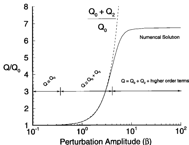
Figure 2. Normalized Q versus perturbation amplitude in the analytical and numerical solutions for the synthetic example.
