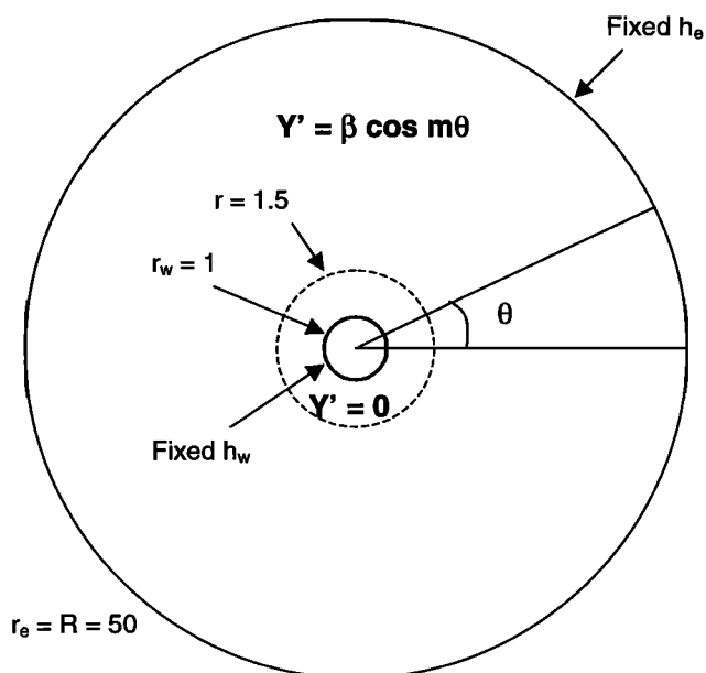
Figure 1. Geometry of the log transmissivity Y field used in the synthetic example; Y_w = 0 , and so, Y = Y' .
