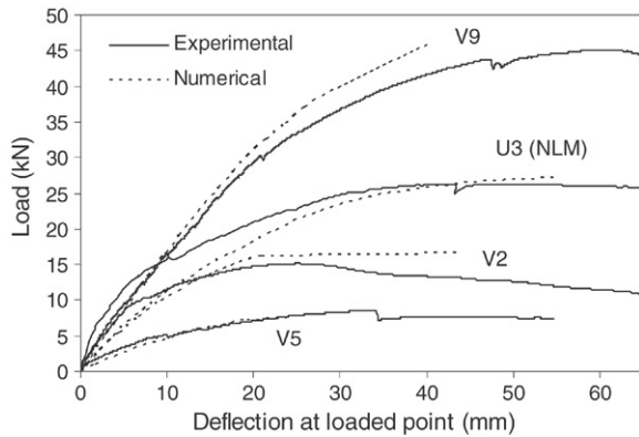
Fig. 10. Load versus vertical deflection experimental and numerical diagrams for vaults U3, V2, V5 and V9.
