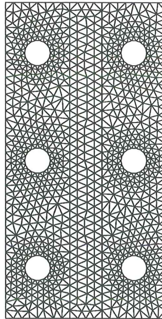
Figure 6: Finite element mesh
