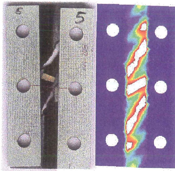
Figure 11: Test of Policinato RS-3 - XN-50 specimen. a) Photograph of tested specimen. b) Equivalent plastic strains contour
