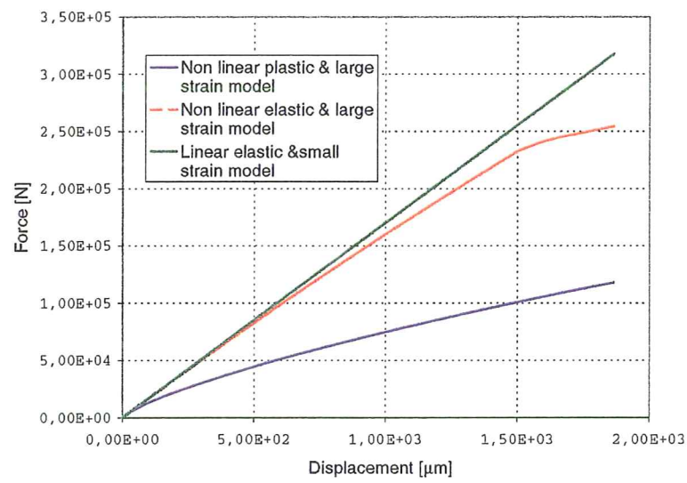
Figure 13: Test of Polycinato RS-3 - XN-50 specimen. Load - displacement plot
