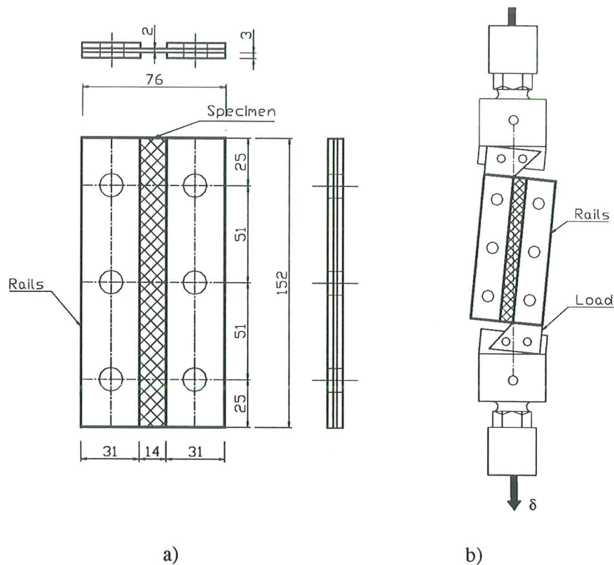
Figure 5: a) Geometry of the specimen b) Testing machine
