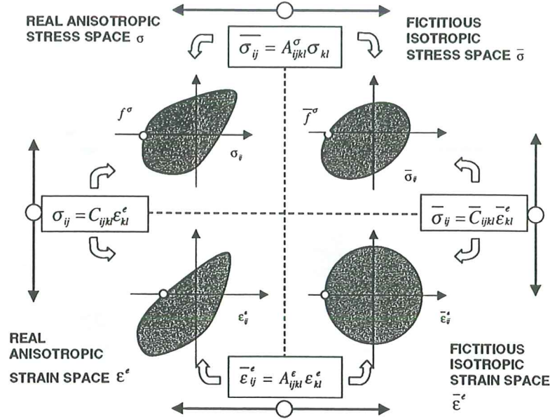
Figure 1: Space transformations. Real and fictitious stress and strain spaces in small strains
