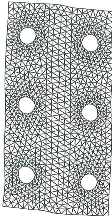
Figure 8: Shear test ASTM D4255. Deformation 3:1
