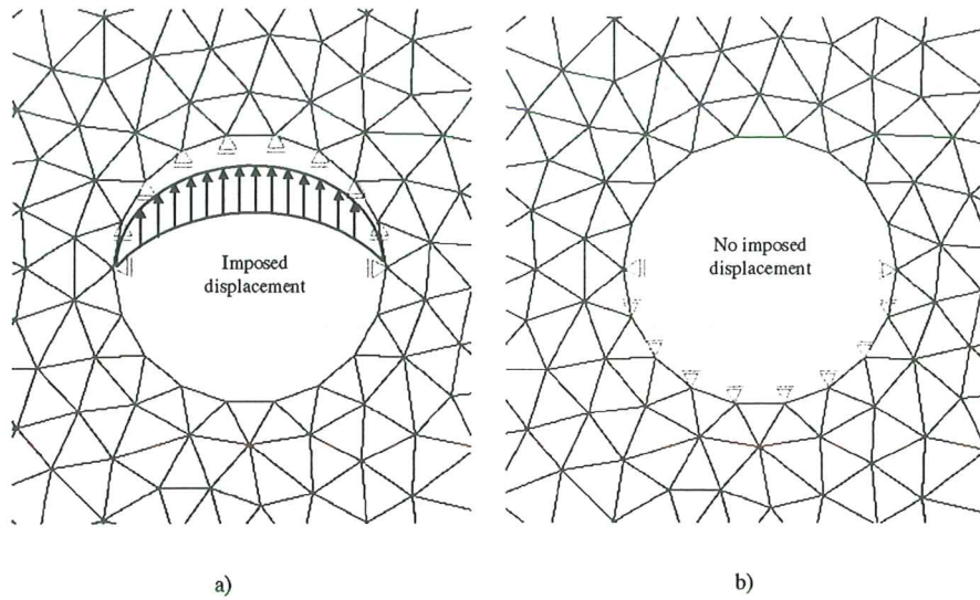
Figure 7: Boundary conditions used in the numerical simulation. a) Left holes. b) Right holes
