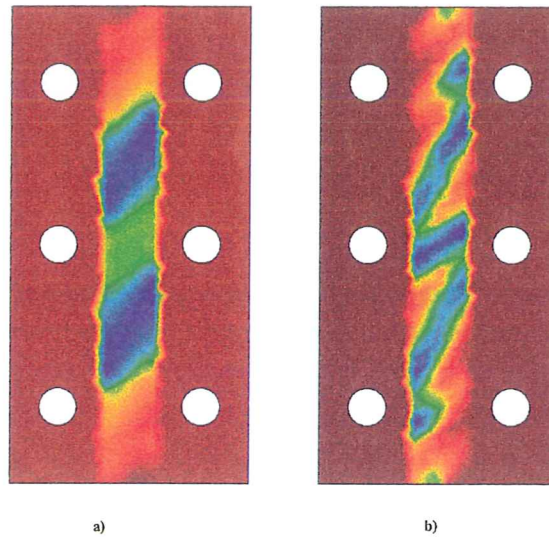
Figure 10: Test of Policinato RS-3 - XN-50 specimen. a) Contour of shear stress \sigma_{xy} b) Contour of plastic shear strains e^p
