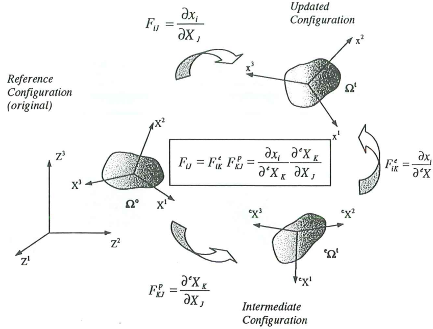
Figure 2: Original, intermediate and deformed configurations
