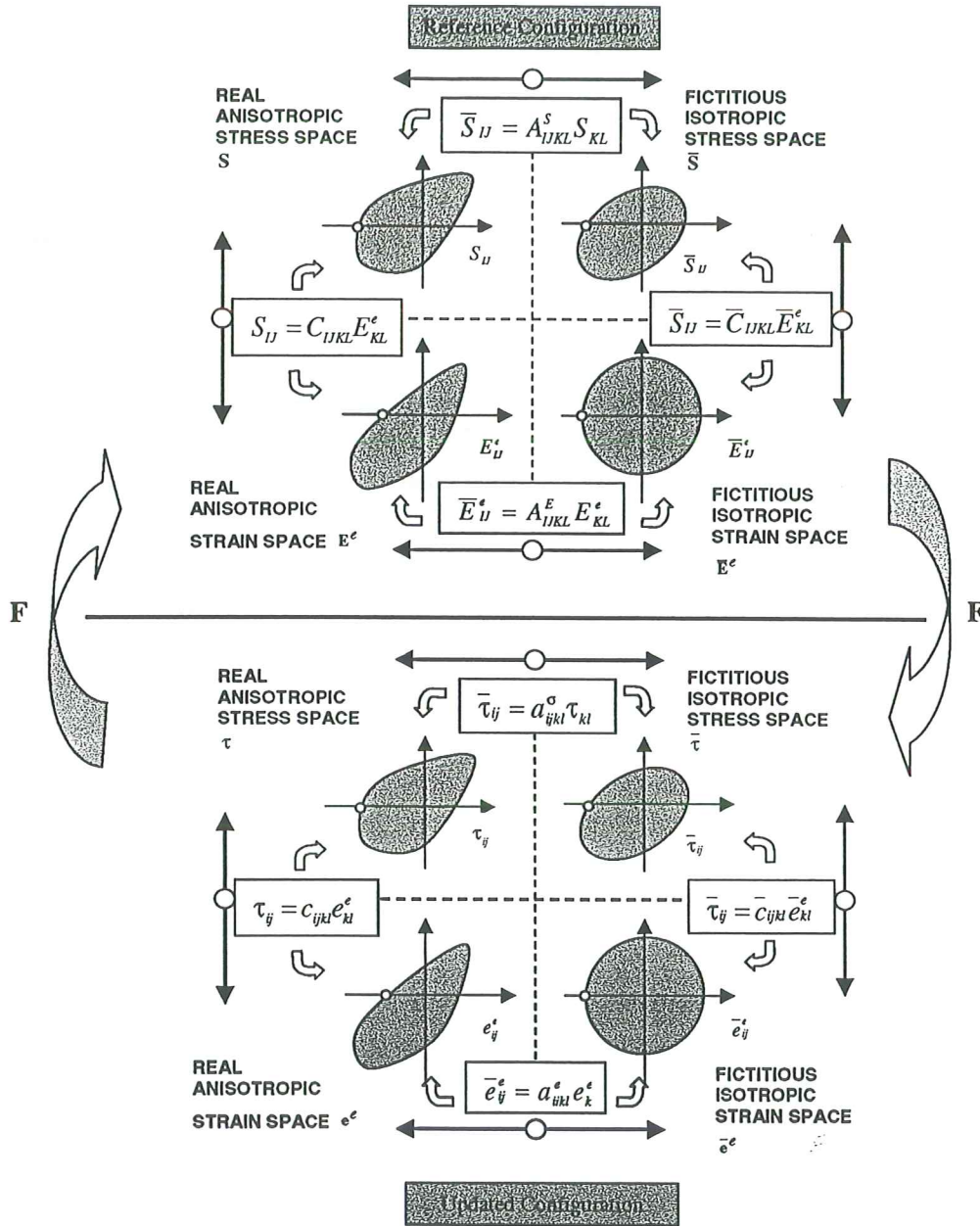
Figure 3: Extension of the anisotropic model to large strains. Spaces definition in reference and updated configurations.
