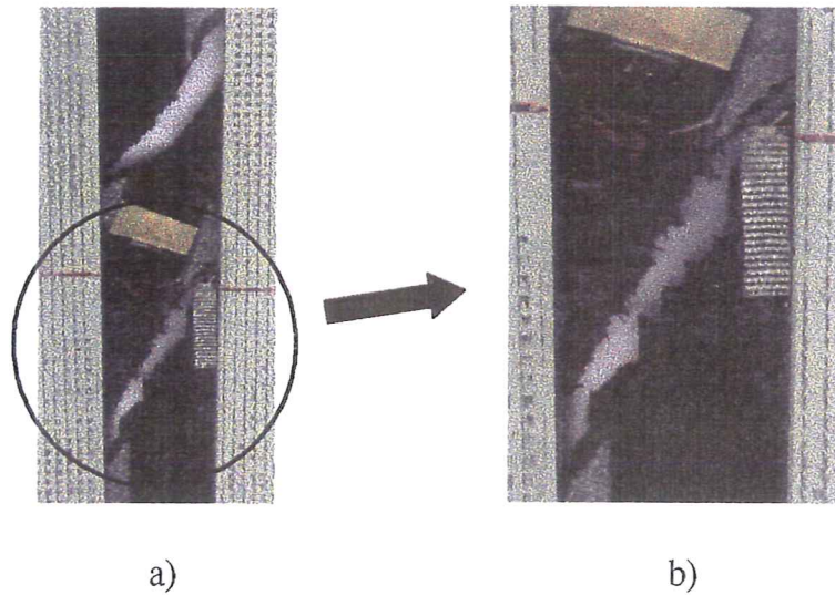
Figure 12: Test of Policinato RS-3 - XN-50 specimen. a) Detail of central area. b) Detail of a crack
