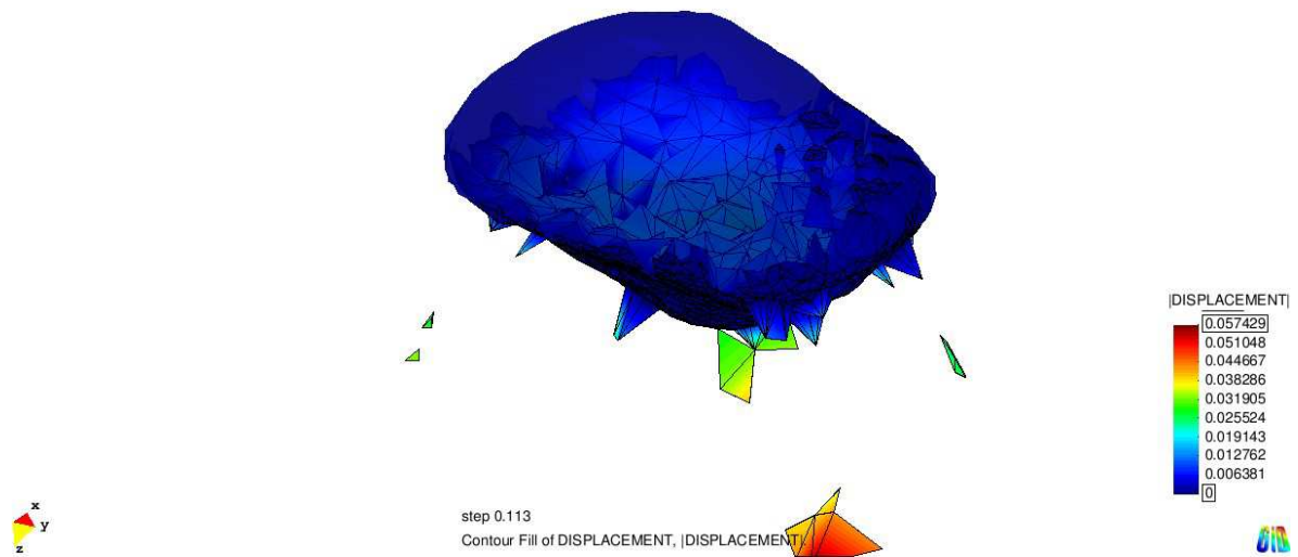
Figure 3.83 – Fluid and structure during at a given time of the voiding process
