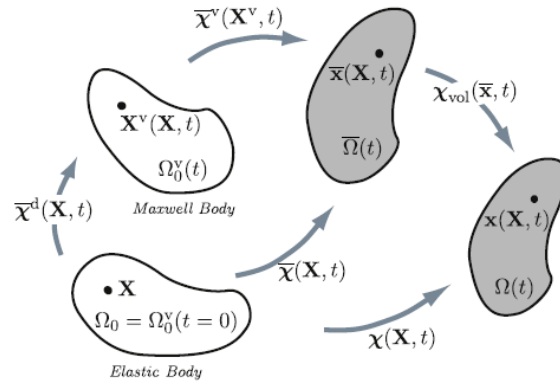
Figure 3.30 –Scheme for the kinematics of the viscoelastic body
