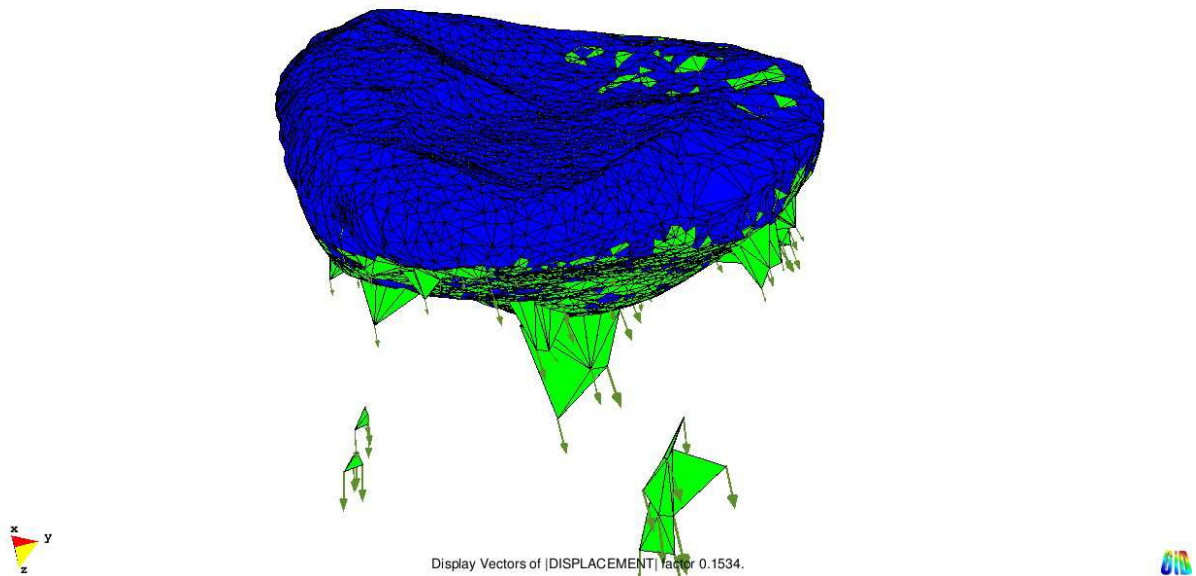
Figure 3.84 – Representation of displacement vectors at a given time of the voiding process
