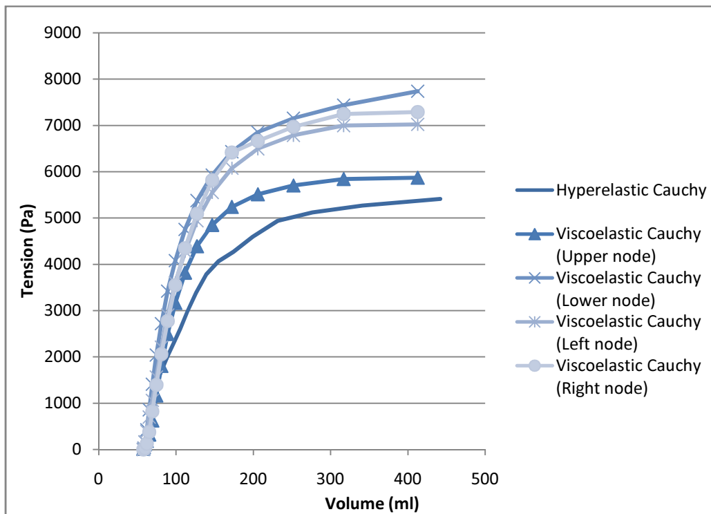
Figure 3.37 – Principal Cauchy stresses vs bladder volume, in four different locations of the bladder
