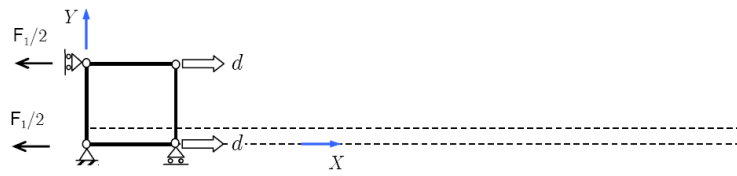
Figure 3.31 – Simple traction test 2D scheme
