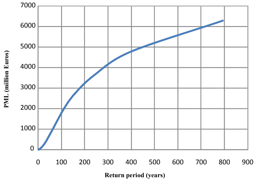
Figure 8. PML curve for Barcelona
