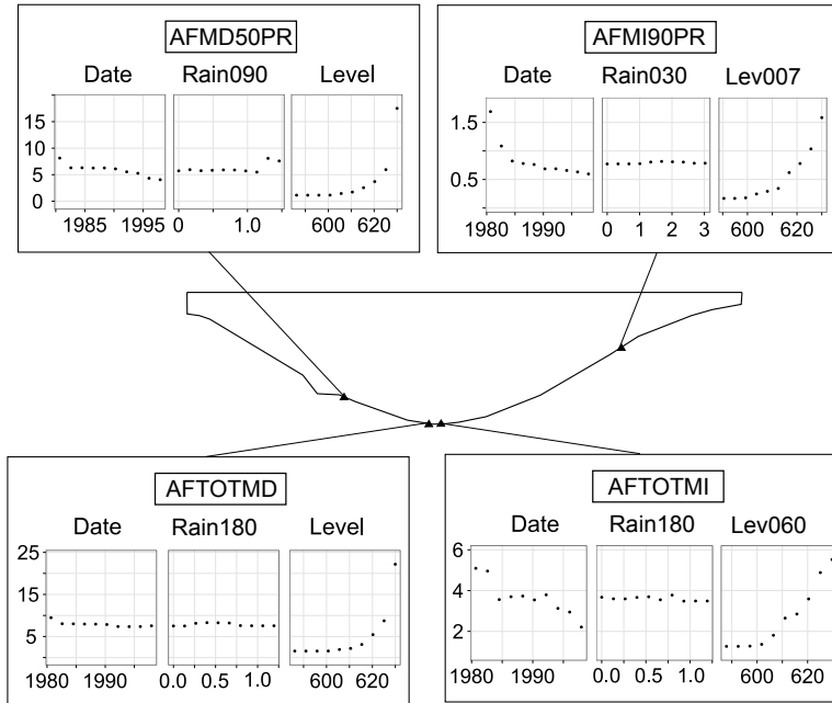
Figure 10: Partial dependence plot for leakage flows.
