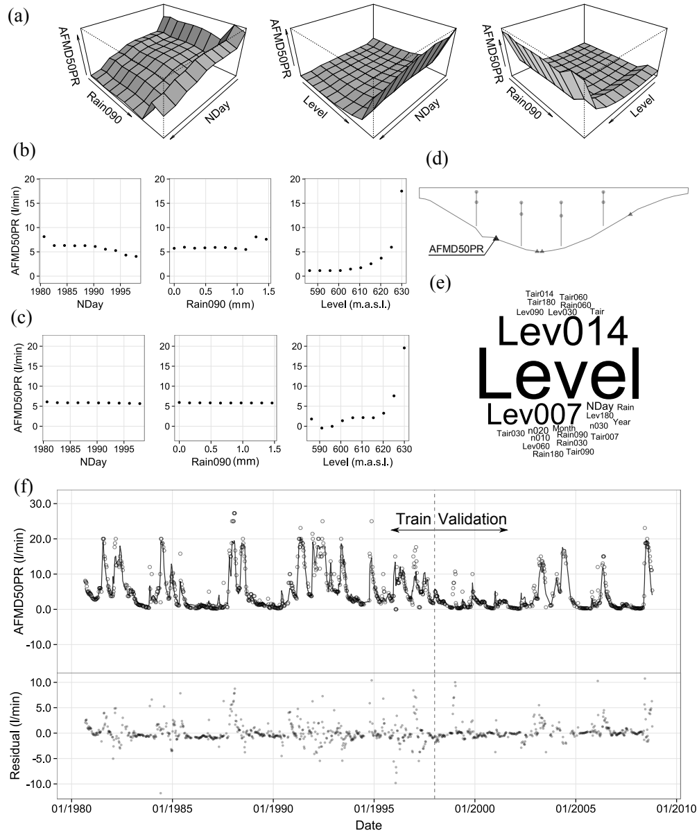
Figure A11: AFMD50PR. (a) 3D partial dependence plot; (b) 2D Partial dependence plot; (c) Idem for artificial data (time-independent); (d) Device location; (e) Word cloud of relative influence; (f) Model fit and residuals for the train and the validation sets.
