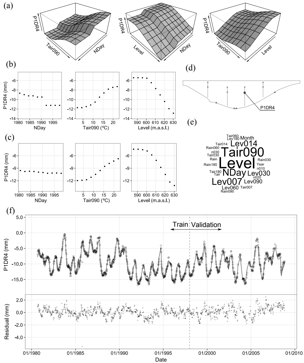
Figure A4: P1DR4. (a) 3D partial dependence plot; (b) 2D Partial dependence plot; (c) Idem for artificial data (time-independent); (d) Device location; (e) Word cloud of relative influence; (f) Model fit and residuals for the train and the validation sets.
