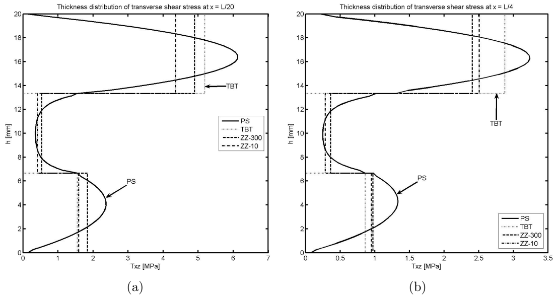
Figure 21: Non symmetric 3-layered SS thick beam under uniformly distributed load ( \lambda = 5 ). Thickness distribution of the shear stress at x = L/20 (a) and at x = L/4 (b)
