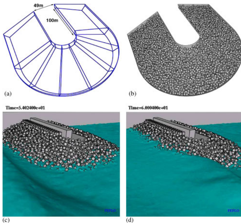
Figure 9. (a, b) Breakwater: domain definition and resulting mesh and (c, d) breakwater: results for a typical simulation.
