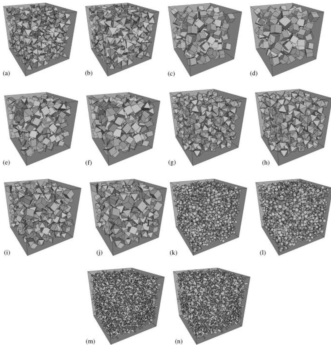
Figure 8. (a, b) Cube filled with tetrahedra; (c, d) cube filled with hexahedra; (e, f) cube filled with prisms; (g, h) cube filled with octahedra; (i, j) cube filled with a mix of objects; (k, l) cube filled with tetrapods (Type I); and (m, n) cube filled with tetrapods (Type II).
