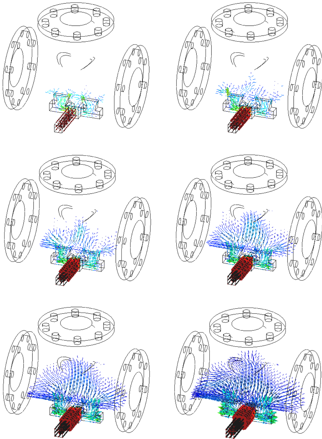
Figure 13: Tee-shape. Velocity vectors along time.
