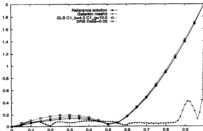
Fig. 5. Velocity variation along the middle section using Q_1 elements ( C_{1b} \equiv C_{1\beta} and C_{1g} \equiv C_{1\gamma} ). The reference solution is computed with \omega = 0 and the Q_1/P_0 element.
