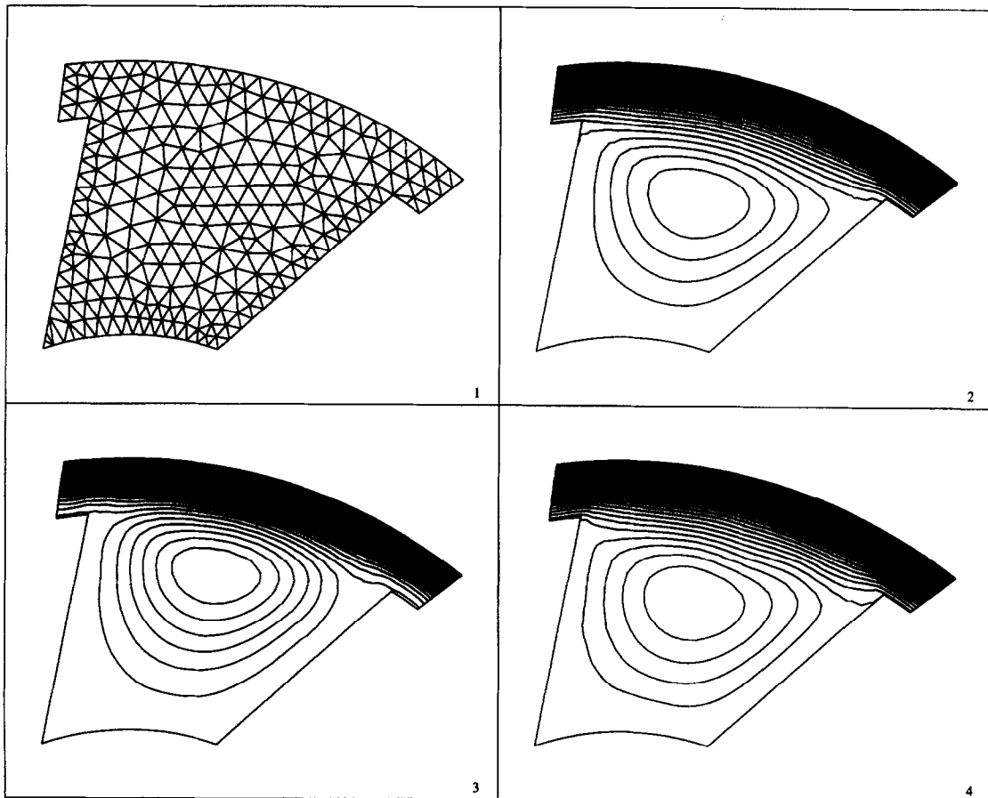
Fig. 12. (1) Unstructured mesh of triangles. (2) Streamlines using the GLS method with P_1 elements. C_{1_\beta} = 1 , C_{1_\gamma} = 10 . Streamfunction peaks: 0.354 and -0.00151 . (3) Streamlines using the GLS method with P_2 elements. C_{1_\beta} = 0.001 , C_{1_\gamma} = 1 . Streamfunction peaks: 0.318 and -0.00534 . (4) Streamlines using the DRS method with P_2^*/P_1 elements. \delta = 0.02 . Streamfunction peaks: 0.372 and -0.000347 .
