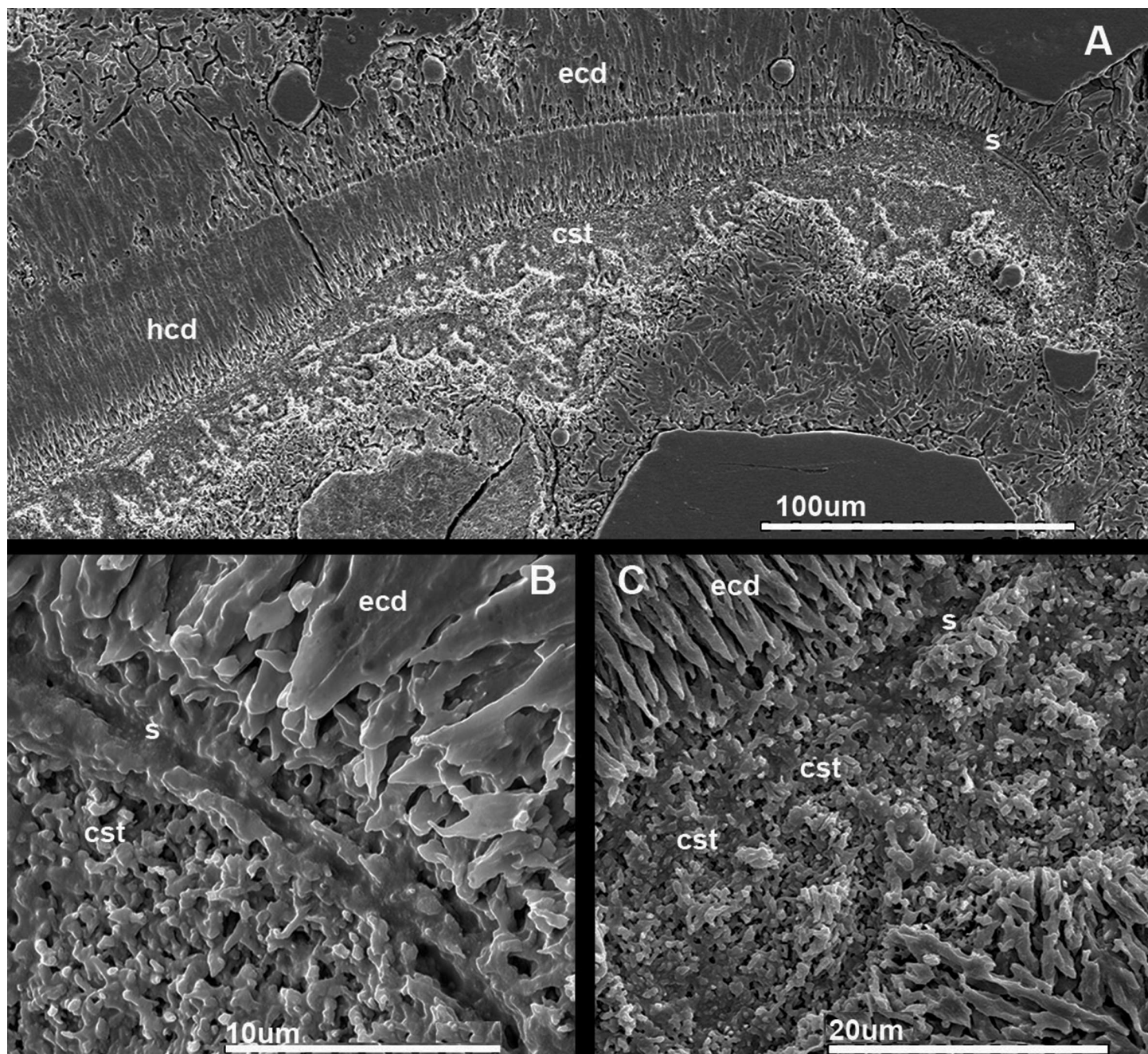
Fig 5. Antarcticeras nordenskjöldi. NRM-PZ Mo 167764. Early Eocene (Ypresian); Seymour Island, Antarctica. Hyposeptal cameral soft tissues. A, general view. B, C, enlargements of A to show a microglobular ultrastructure of cameral soft tissues, median shell section. Cst, cameral soft tissue; ecd, episeptal cameral deposits; hcd, hyposeptal cameral deposits.
