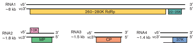
Fig. 2. Genome organization of the genus Ophiovirus . Mirafiori lettuce big-vein virus is shown (modified from [2]). Boxes represent ORFs. The length of the RNA segments and the predicted sizes of the ORF products are indicated. RNA4 is not reported for all ophioviruses. v, viral RNA; vc, viral complementary RNA; RdRp, RNA polymerase; MP, movement protein; CP, coat protein.
