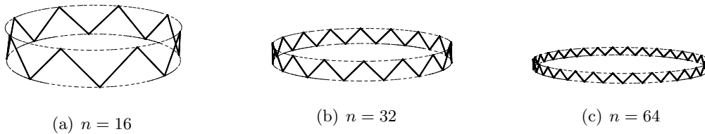
Figure 1. Examples of the contour for n = 16, 32 and 64 . The polygon is formed by connecting with light-like lines two sets of points lying on a circle at t = 0 and at t = 2 \sin \frac{\pi}{n} respectively ( t is the vertical axis in the figures). In the limit n \rightarrow \infty the contour becomes a space-like circle of radius 1.
