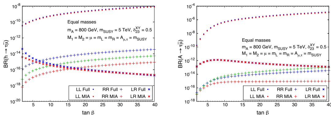
Figure 9. BR(h \rightarrow \tau\bar{\mu}) (left panel) and BR(A \rightarrow \tau\bar{\mu}) (right panel) as functions of \tan\beta in the Equal masses scenario with m_{\text{SUSY}} = 5 TeV, m_A = 800 GeV, and \delta_{23}^{XY} = 0.5 , with XY = LL, RR, LR ( \tilde{\delta} , for the latter), in each case. The green crosses are the MIA predictions in the RR case after including the \mathcal{O}(M_W^2/m_{\text{SUSY}}^2) corrections. The results for the heavy scalar H (not shown) are nearly equal to these ones for the pseudoscalar A .
