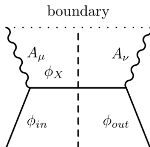
Figure 2. Witten diagram representing the s -channel contribution to the holographic dual description of FCS in the N \rightarrow \infty limit. The vertical dashed line schematically represents the optical theorem procedure used to extract the relevant imaginary part of T^{\mu\nu} . There is a single-hadron intermediate state, which means that only single-hadron final states are considered in DIS. The horizontal dotted line represents the boundary of \text{AdS}_5 . In addition, \phi_{in} , \phi_X and \phi_{out} are the dual supergravity fields of the initial, intermediate and final hadronic states, respectively, while A_\mu couples to J^\mu of the quantum field theory at the AdS boundary.
