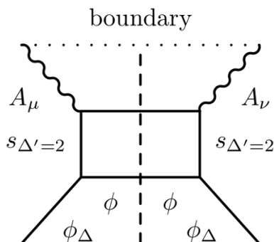
Figure 4. Witten diagram corresponding to the one-loop dominant contribution to FCS.
